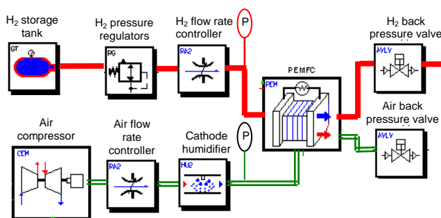
Fig. 1. Simplified scheme of the fuel cell testbench
