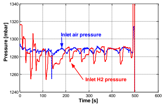
Fig. 2d. Evolution of the gas pressures at stack inlets
