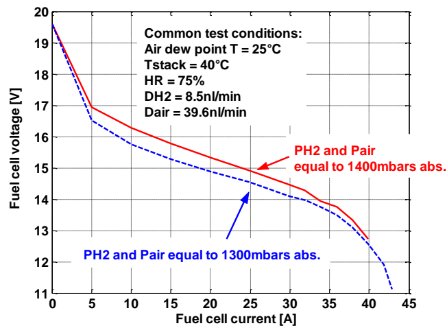
Fig. 4. Polarisation curves recorded for two hydrogen and air pressures
