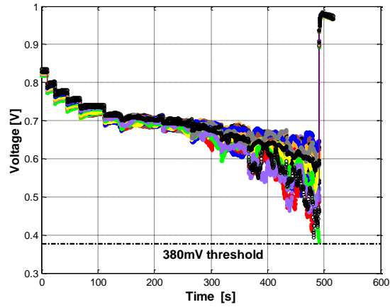
Fig. 2b. Evolution of the 20 cell voltages
