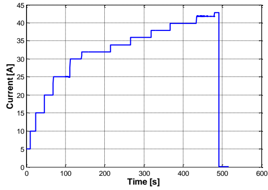
Fig. 2a. Evolution of the FC current
