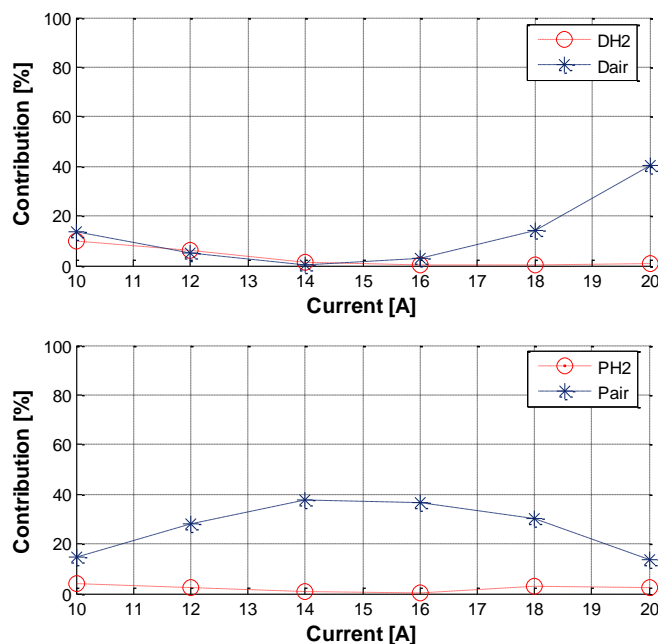
Fig. 5. Contribution of the four studied parameters to the FC voltage
