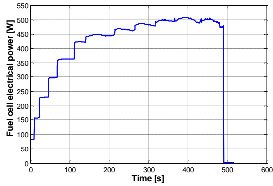
Fig. 2c. Evolution of the FC stack power
