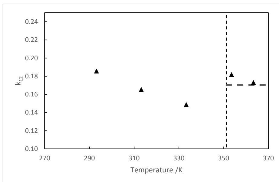
Figure 6: k_{12} binary parameter as a function of temperature. Vertical dashed line: R32 critical temperature. Horizontal dashed line: parameter value obtained after considering all the data for T > T_c(\text{R32}) .
