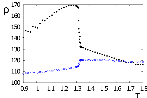
Figure 8. Variable \rho as a function of T for \eta = 0.26 with D_1 = 0.8 (black circles) and D_1 = 1 (blue open circles). We have used N_x = N_y = 20, N_z = 6, I_0 = K_0 = 0.5, D_2 = 1, D = 1 and \epsilon = 1 . See text for comments.
