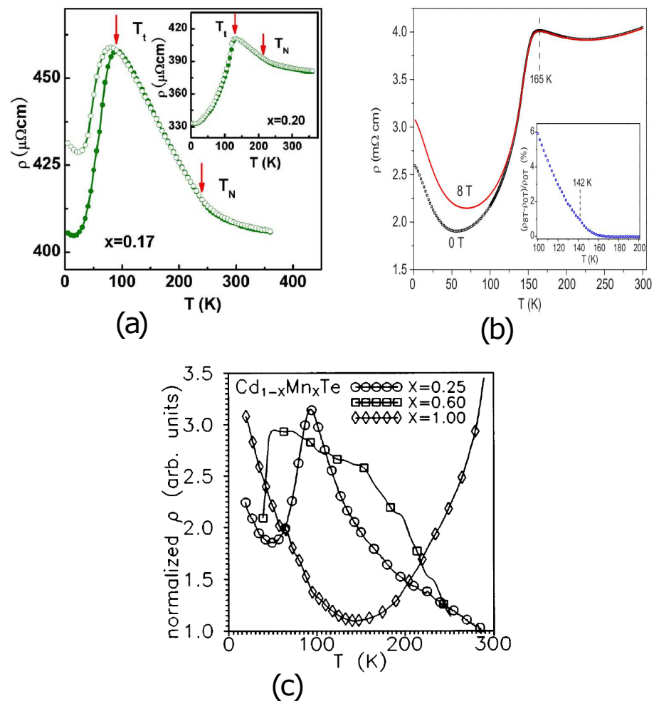
Figure 19. Experiments on the resistivity as a function of T performed by (a) by Du et al. on \varepsilon -( Mn_{1-x}Fe_x ) 3.25 Ge antiferromagnets [3], (b) by McGuire et al. on antiferromagnets LaFeAsO [6] and (c) by Chandra et al. on thin films of Cd 1-x Mn x Te [39].
