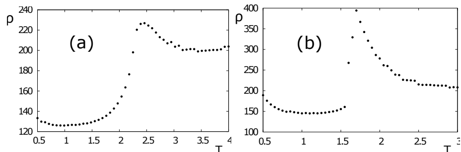
Figure 18. Spin resistivity \rho of the Ising HCP model versus temperature T for (a) \eta = 0.3 ; (b) \eta = 1 . N_x = N_y = 18, N_z = 8 (namely 16 planes in the z direction), D_1 = D_2 = 1, \epsilon = 1, I_0 = 2, K_0 = 0.5, C_1 = C_2 = 1, A = 1, D = 0.5 . All distances are in units of the NN distance; energy constants are in units of |J_2| = 1 . See text for comments.
