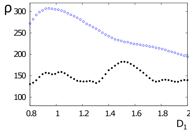
Figure 17. Values for \rho versus D_1 for \eta = 1 at T = 1.5 < T_C (black circles) and at T = 1.9 > T_C (open circles) where T_C \simeq 1.7 . Other parameters are N_x = N_y = 18, N_z = 8, D_2 = 1, I_0 = 2, K_0 = 0.5, C_1 = C_2 = 1, A = 1, D = 0.5 and \epsilon = 1 .
