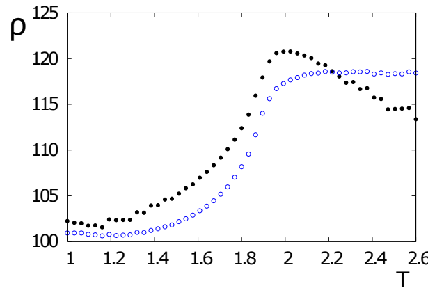
Figure 7. Variable \rho as a function of T for \eta = 0.2 with D_1 = 0.8 and 1 (black circles and blue open circles, respectively). For simulations, we used N_x = N_y = 20, N_z = 6, I_0 = K_0 = 0.5, D_2 = 1, D = 1 and \epsilon = 1 .
