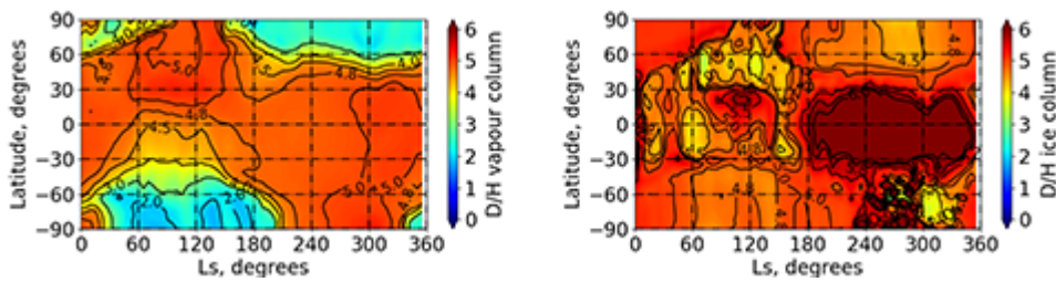
Figure 1: Zonal mean of the integrated column of D/H vapor and ice ratio over a martian year at the 10^0 Ls (Solar Longitude). GCM simulation run with the radiative active water ice clouds and the microphysics
