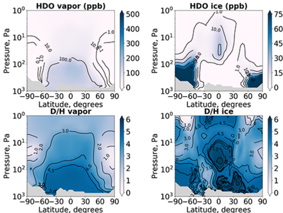
Figure 2: Zonal mean cross sections of HDO vapor, HDO ice, D/H vapor and D/H ice during southern sp
