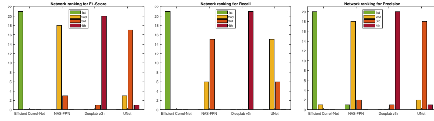
Fig. 4: Rankings of the different networks (from left to right: Efficient Correl-Net , NAS-FPN, Deeplab v3+, U-Net) for each scene of the DAVIS test dataset, regarding the metrics (from left to right: F1-Score, Recall, Precision).
