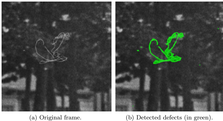
Fig. 1: Detection of defects (1b) in an old film frame (1a) with Efficient Correl-Net .
