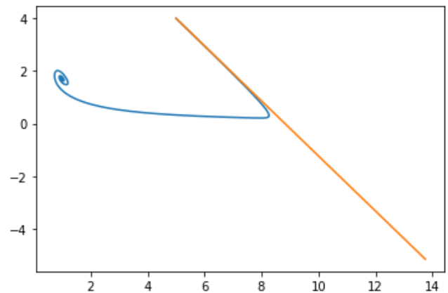
Figure 3: Single-step simulation with h = 0.1
