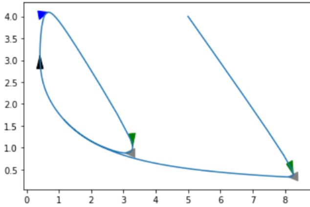
Figure 4: Our approach on 280 steps
