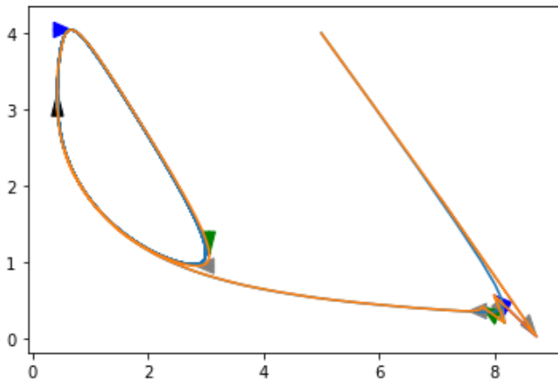
Figure 8: Proximity adaptation only.
