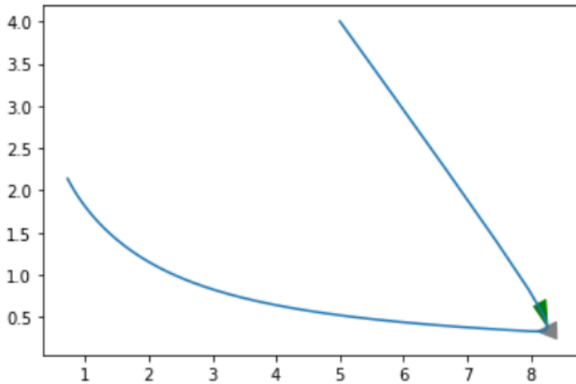
Figure 5: Fixed integration step (0.01) on 280 steps
