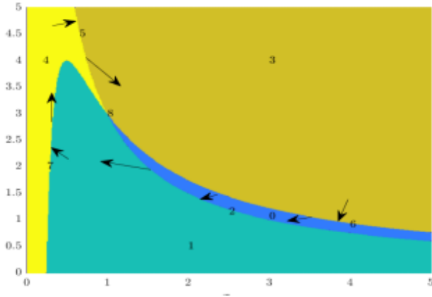
Figure 1: Qualitative state space for a Brusselator
