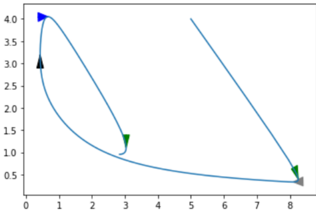
Figure 6: Fixed integration step (0.01) on 800 steps.
