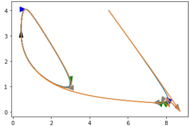
Figure 7: Fixed integration step of 0.025 and false transitions
