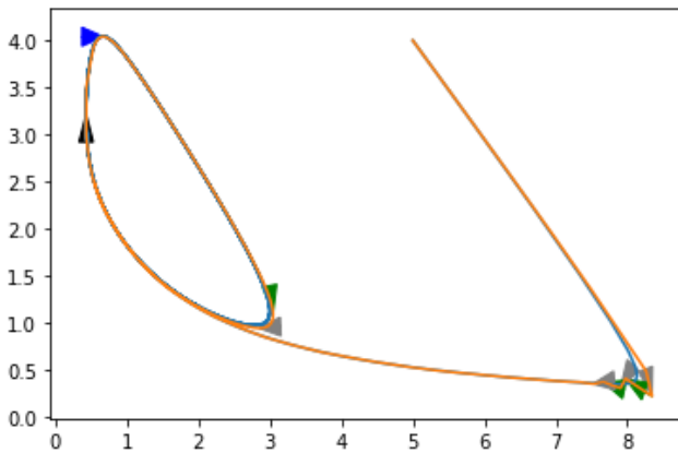
Figure 9: Variation adaptation only.
