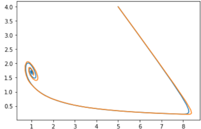
Figure 2: Our results (orange) vs. real behavior (blue)
