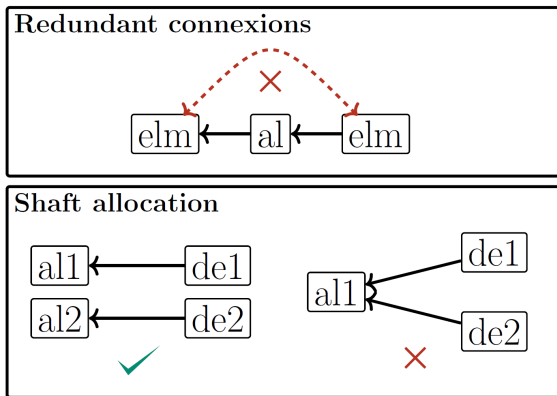
Figure 2: Constraints on redundant connection and shaft allocation
