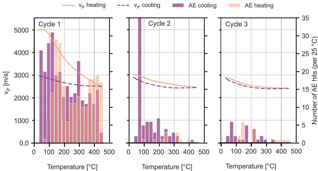
Figure 10. Passive and active acoustic monitoring of Westerly granite during thermal stressing: P -wave velocity ( v_p ) and number of acoustic emissions detected during three cycles of heating and cooling to a peak temperature of 450°C (data from Griffiths et al. (2018)).
