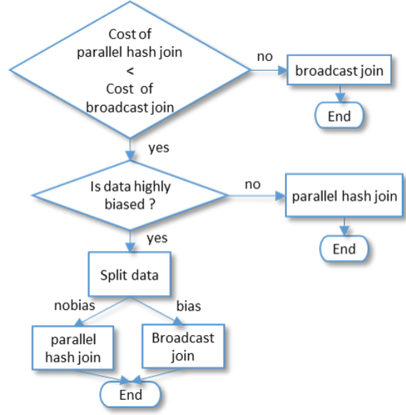
Figure 4: Physical join operation selection
