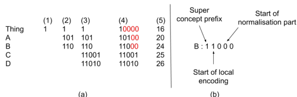
Figure 2: LiteMat encoding example
