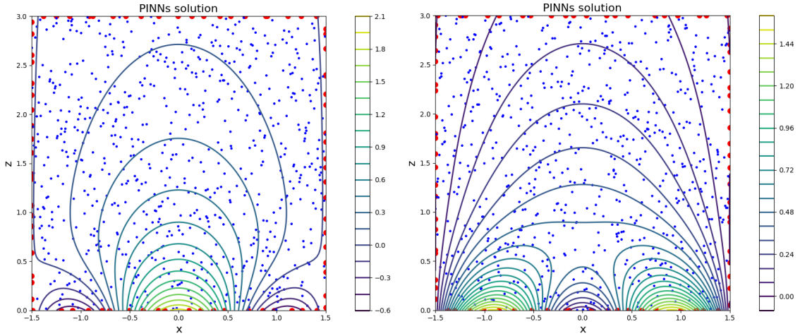
Figure 17: Solutions (iso-contours of u(x, z) ) predicted by PINNs solver for the Helmholtz equation for two cases, i.e. for the parameters combination (a_1, a_2, a_3) equal to (1, 0, 1) and (1, 0, -1) in left and right panel respectively. The distribution of data sets (training and collocation points) is also indicated using red and blue dots at the boundary and inside the domain respectively.
