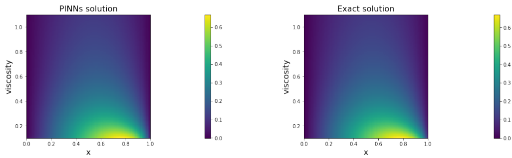
Figure 31: Colored iso-contours of the predicted PINNs solution u(x, \mu) and exact solution in the left and right panel respectively.
