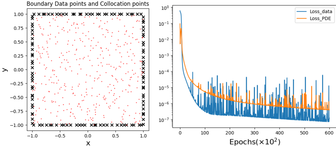
Figure 6: (Left panel) Distribution of data sets showing the space localization of training data points at the four boundaries (i.e. N_{data} = 120 ) and collocation points (i.e. N_c = 400 ) inside the domain, for solving Laplace problem using vanilla-PINNs. (Right panel) Evolution of the two partial losses L_{data} and L_{PDE} as functions of the number of iterations (i.e. epochs).
