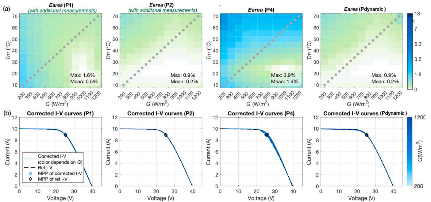
Fig. 7. (a) Heatmap for the area error of the correction of I-V curves under the R_s degradation using P1, P2 (with additional I-V curves), P4, and Pdynamic (gray points represent the G and T_m of I-V curves shown below); (b) Examples of corrected I-V curves whose parameters G and T_m are distributed along the diagonal of the heatmap in (a). P2 and Pdynamic exhibit similar good performance but P1 and P2 require additional I-V curves to obtain r_s coefficient. (For interpretation of the references to colour in this figure legend, the reader is referred to the Web version of this article.)
