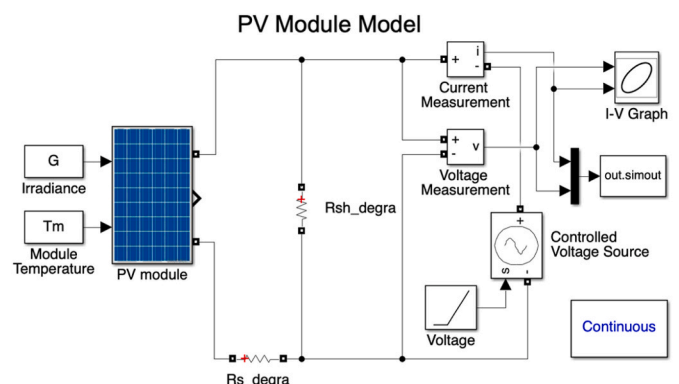
Fig. 1. Simulation model of the PV module under Matlab Simulink.
