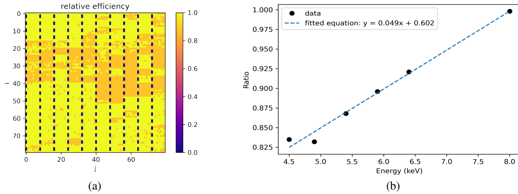
Fig. 3. Three pixel populations found in the ECLAIRs detection plane (left: HTPs in black, LEPs in orange, and HEPs in yellow). The ratio of the mean number of relative counts between the LEP and the HEP as a function of energy is shown on the right, and it is fit with a linear function.
