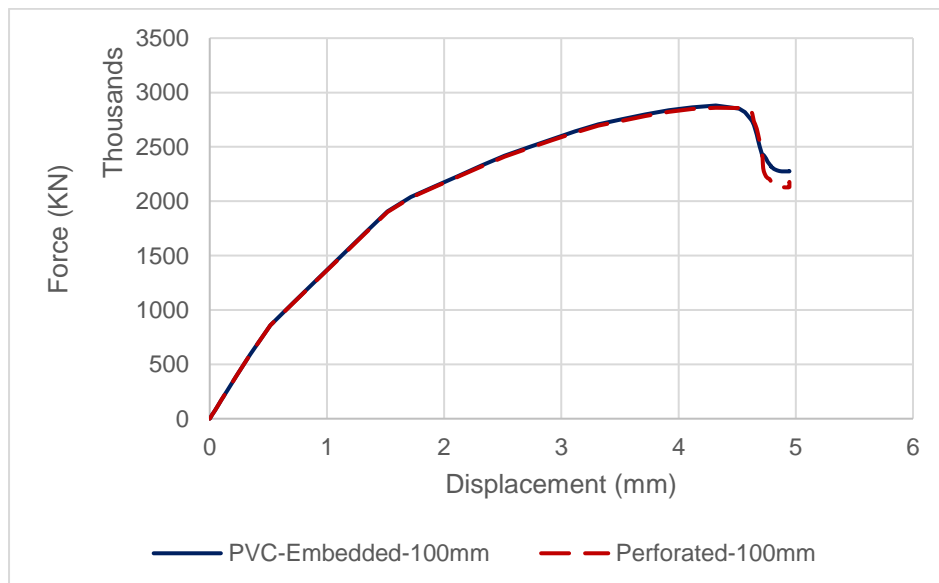
Fig. 11. Force-displacement relationship of PVC embedded columns and perforated columns without PVC
