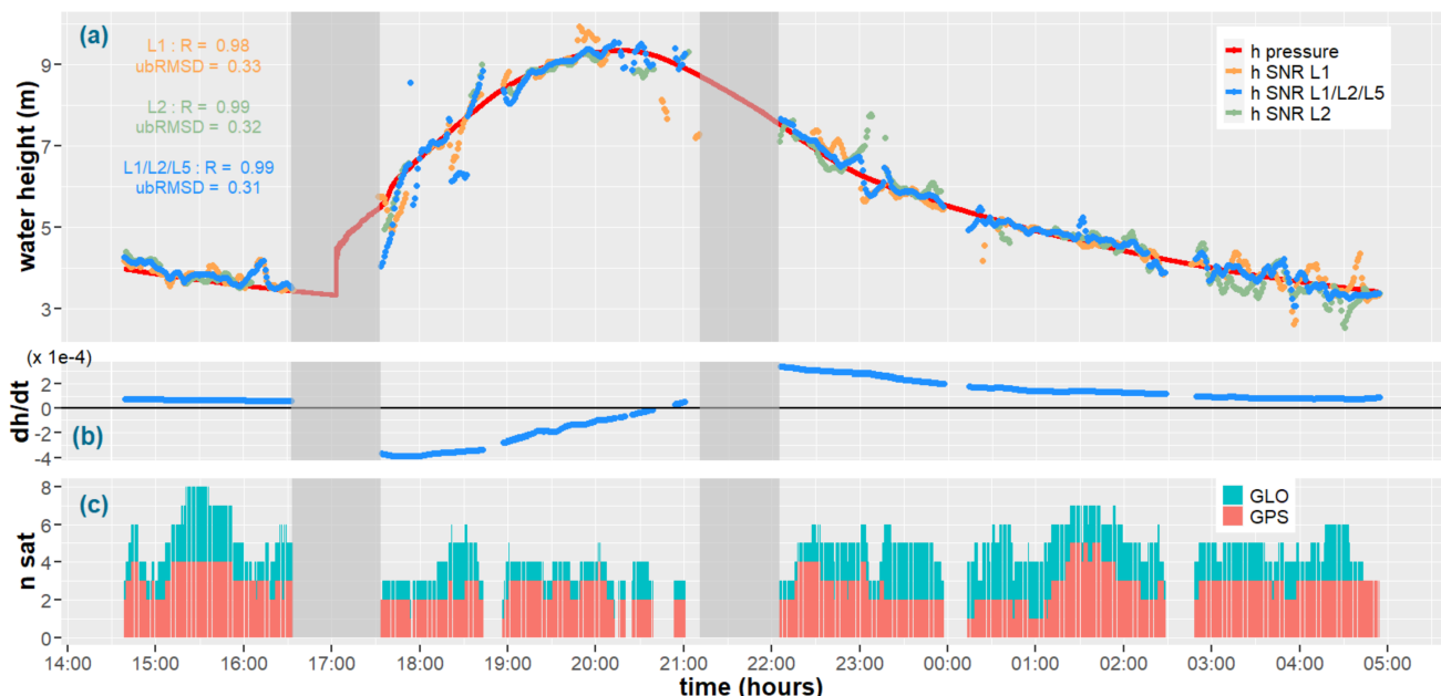
Figure 5. Final results using the adapted dynamic SNR inversion. (a) Comparison of h calculated using L1 only (orange), L2 only (green), and L1 + L2 + L5 (blue) frequencies for GPS and GLONASS satellites with pressure water levels (red); (b) output \dot{h} with L1 + L2 + L5 bands; (c) number of GPS and GLONASS satellites for the calculation of h and \dot{h} . The value of \dot{h} was derived from the relative antenna height h , thus it was negative during rising tides as the relative antenna height decreased.
