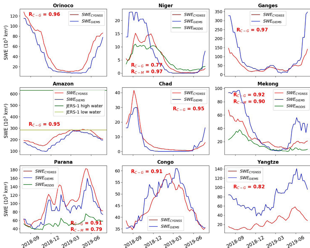
Fig. 11. Time series of weekly surface water extent estimated from CYGNSS and GIEMS (upsampled from the 10-day GIEMS product), averaged for 9 River basins: (a) Orinoco, (b) Amazon, (c) Parana/La Plata, (d) IND, (e) Chad (f), Congo, (g) Ganges-Brahmaputra, (h) LMB, and (i) Yangtze. Also shown, the MODIS surface water extent time series for the Parana, IND and LMB, and the surface water extent at high and low water stages in the Amazon from Hess et al. (2015). The correlations between the time series of SWE_{CYGNSS} and SWE_{GIEMS} ( R_{C-G} ) and, when exist, SWE_{MODIS} ( R_{C-M} ), are printed in red in each subplot. (For interpretation of the references to color in this figure legend, the reader is referred to the web version of this article.)
