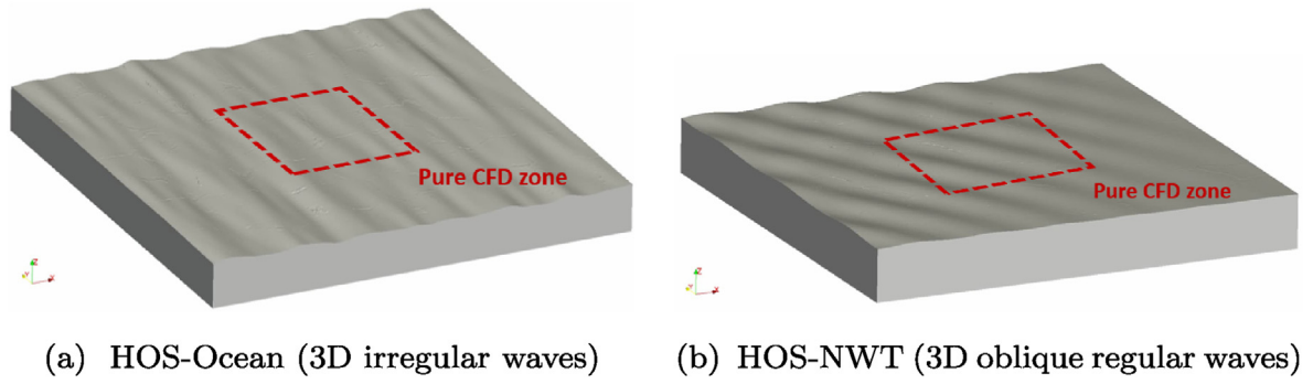
Fig. 9. Simulated HOS wave fields in CFD.
