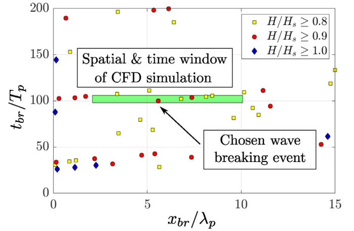
Fig. 12. Wave-breaking events identified during the HOS simulation and the chosen temporal and spatial window for the CFD simulation.
