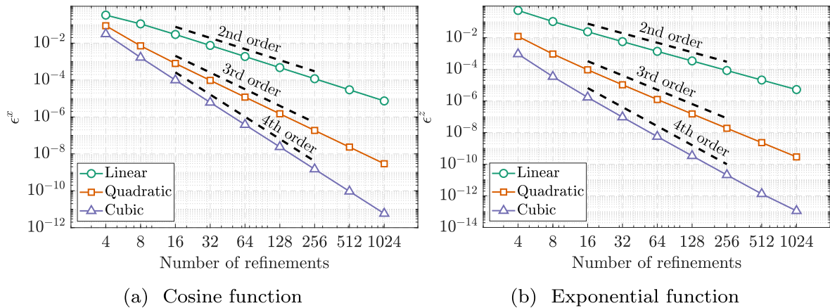
Fig. 3. Interpolation errors with respect to refinement for two test functions.
