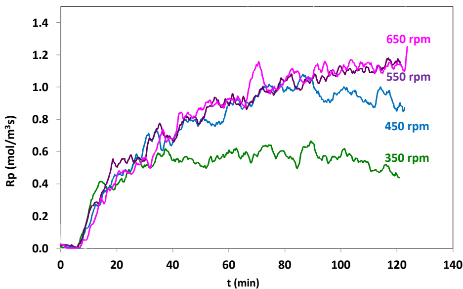
Figure 9. Polymerization rate for different agitation speeds (setup S2+D).
