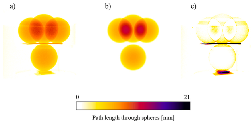
Fig. 4. Measurement of three-dimensional ball positions using radiographs. a) shows the original radiograph after calibration, b) presents a synthetic radiograph generated with the measured ball positions, and c) displays the residual of correlations between the two images. The scale refers to a) and b), with the same color-code applied for the residual's value (in mm 2 ) in c). (For interpretation of the references to color in this figure legend, the reader is referred to the Web version of this article.)
