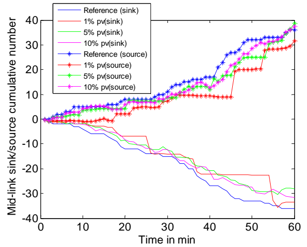
Figure 12. Cumulative number of mid-link sink/source with 5% perturbation.
