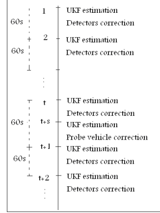
Figure 2. UKF algorithm.
