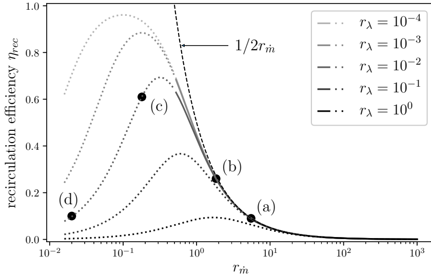
Figure 3.: Recirculation efficiency \eta_{rec} for various values of the dimensionless parameters r_{\dot{m}} and r_\lambda . Solid lines: r_{\dot{m}} > 0.5 and r_{\dot{m}}/r_\lambda > 50 . Dotted lines: r_{\dot{m}} < 0.5 or r_{\dot{m}}/r_\lambda < 50 . The points (a-d) correspond to Figure 2.
