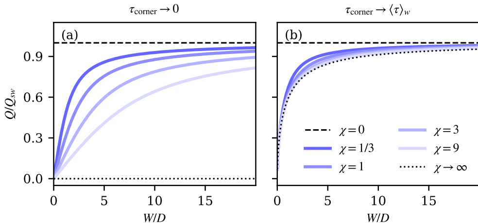
Figure 7: The water discharge, Q , normalised by the shallow-water discharge, Q_{sw} = WD\sqrt{gSD/C_f} , in rectangular channels as a function of the channel's aspect ratio, W/D , in the case of (a) \theta = 0 , and (b) \theta = 1 . Different colors stand for different values of \chi . The black dashed line corresponds to the shallow-water theory ( \chi = 0 ), while the black dotted line corresponds to the high-diffusion theory ( \chi \rightarrow \infty , equation 5.8).
