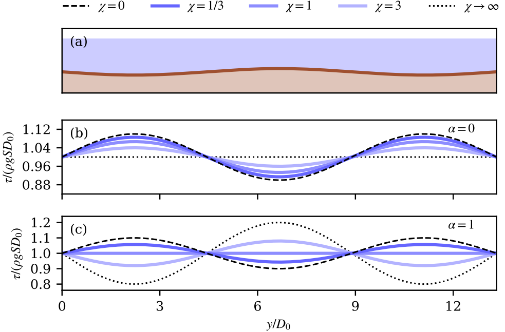
Figure 8: (a) An infinitely wide channel with a wavy bottom (equation 5.9), with \delta/D_0 = 0.1 and D_0k = 1/\sqrt{2} . (b) Stress distribution of equation 5.10 with \alpha = 0 . Different colored lines stand for different values of \chi . The black dashed line stands for the shallow-water theory, \tau(y) = \rho g S D(y) ( \chi = 0 ), while the black dotted line stands for the high diffusion limit ( \chi \rightarrow \infty ). (c) Stress distribution of equation 5.10 with \alpha = 1 . The dark blue curve corresponds to the laminar flow ( \chi = 1/3 and \alpha = 1 ). The value \chi = 1 is the critical value beyond which the stress distribution inverts.
