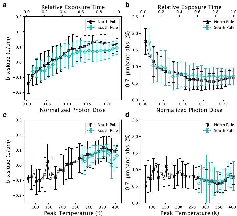
Fig. 6 Comparison between observed spectrophotometric indexes and modeled values. a b-x slope value versus normalized photon dose. b 0.7- \mu\text{m} band absorption versus normalized photon dose. c b-x slope value versus peak temperature at perihelion. d 0.7- \mu\text{m} band absorption versus peak temperature at perihelion. The north polar observation (Fig. 1a) and the south pole observation (Fig. 1c) are shown with black and cyan markers, respectively. Observed spectrophotometric indexes are binned by every 0.1 for photon dose and every 10 K for peak temperature. Error bars indicate the standard deviation in each bin. Relative exposure time for a , b is calculated such that the most irradiated surface is defined as unity. Image ids used for this figure are listed in Supplementary Table 1.
