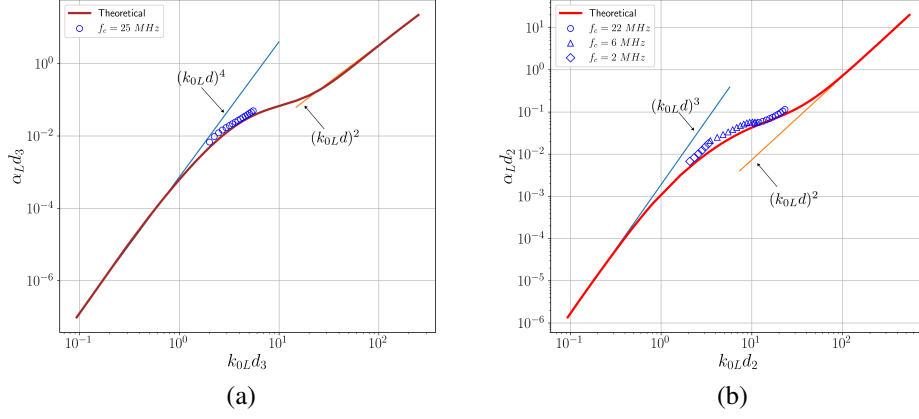
Figure 4: Numerical and theoretical normalized attenuation curves comparison for (a) 3D grain with a_3 = 5a_2 = 5a_1 and (b) 2D grain with a_2 = 5a_1 .
