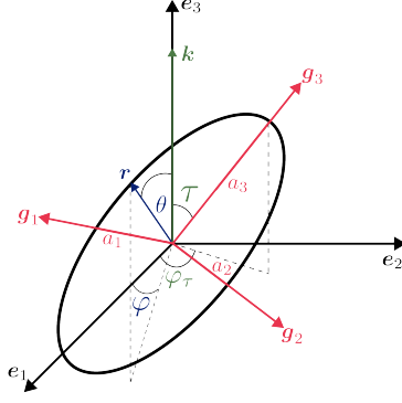
Figure 1: Illustration of an ellipsoidal grain, where a_1, a_2, a_3 are the ellipsoidal radii and \tau, \phi_\tau are the orientation angles of the ellipsoid principal axis g_3 and \theta, \phi are the angles of the vector r .
