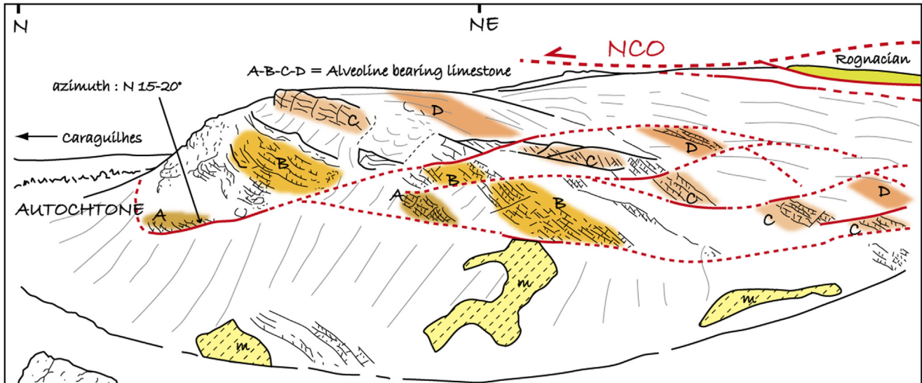
Fig. 4. View of the “Plateau de Poursan” illustrating the development of extensional listric faults developed in the footwall of the NCO. The “Rognacian” allochthonous block is associated with a big Aptian block, which is not visible on the drawing (see the Figs. 1 and 3). m: Miocene formations. The landscape, redrawn from Ellenberger (1967), is no longer visible today due to the vegetation growth.
