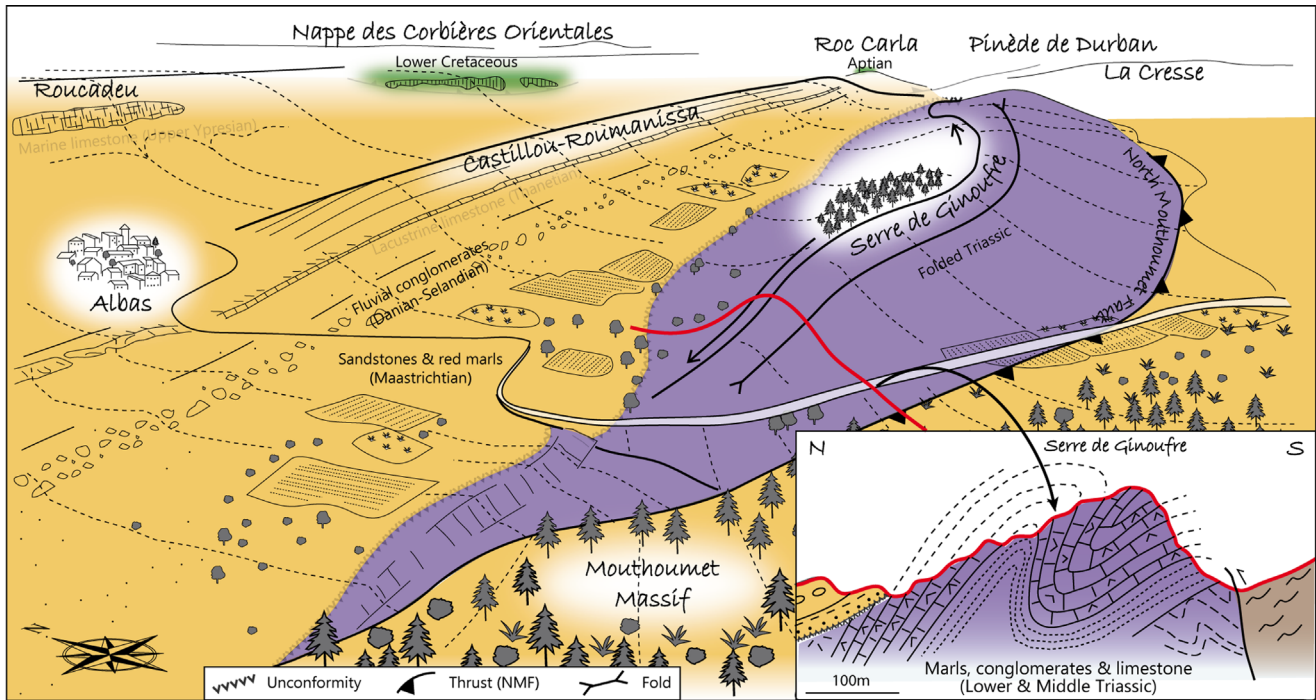
Fig. 6. Geology of the “Serre de Ginoufre”, showing the unconformity between the Garumnian series (north) and the front of the North Mouthoumet Fault (south). The geological section of the “Serre de Ginoufre” demonstrates an ante-Paleogene deformation with the development of East-West folds in the Triassic series. See Figure 3 for the location.
