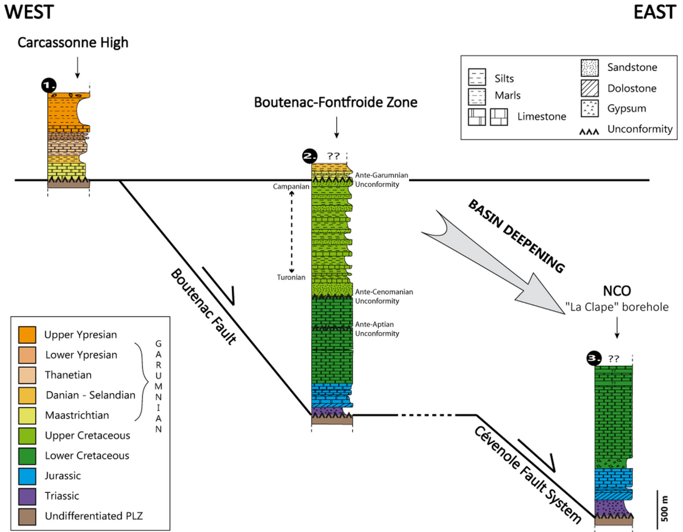
Fig. 2. Generalized litho-stratigraphical logs of the three paleogeographic sectors (Carcassonne High, Boutenac-Fontfroide Zone and the Nappe des Corbières Orientales) showing the eastward deepening of the basin (see Fig. 1 for the location of these zones). After Narbonne and Capendu BRGM 1/50 000 geological notes (Lespinasse, 1982; Ellenberger et al. , 1987). Both Carcassonne High and Boutenac-Fontfroide Zone belong to the eastern Pyrenean foreland, the NCO belongs to the Corbières-Languedoc Transfer Zone (CLTZ).
