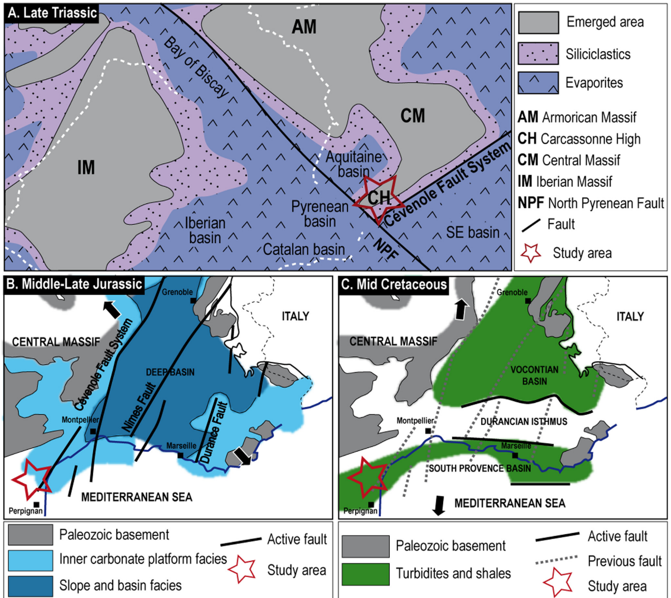
Fig. 8. A. Paleogeographic context of western Europe during the Late Triassic period. The dotted lines correspond to the current boundary between Spain and France. Modified after Orti et al. (2017) . B. and C. Paleogeographic context of the Southeast Basin and faults activity during the Middle-Late Jurassic (B) and Mid Cretaceous (C). Modified after Debrand-Passard (1984) .
