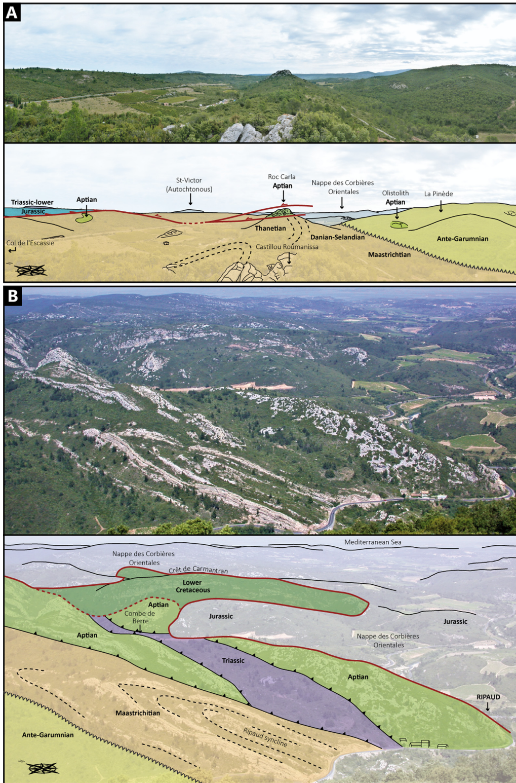
Fig. 5. A. View and interpretation of the “Roc Carla”, from Castellou-Roumanissa hill looking to the east, showing the NW progression of the NCO and the overturning of its footwall. The “Roc Carla” is interpreted as an Aptian block, dragged under the NCO. See Figure 3 for the location. B. View and interpretation of the Ripaud syncline and Combe de Berre, from the Mont St-Victor looking to the east (see Fig. 3 for the location).
