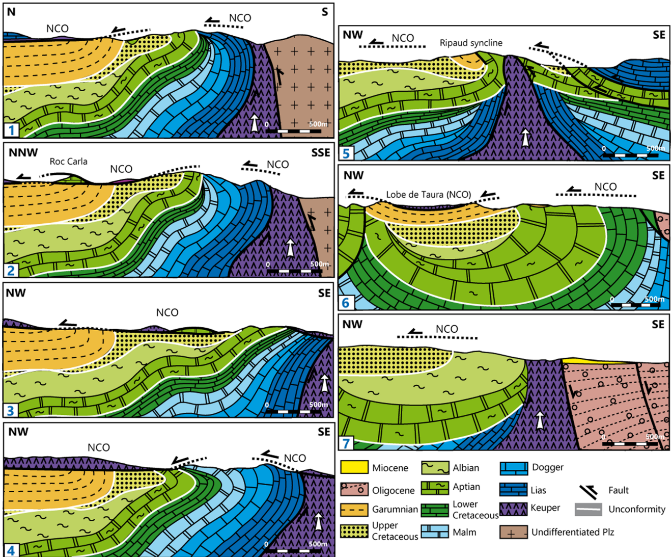
Fig. 7. Geological sections through the “Pinède de Durban” from West (1) to East (4) and geological sections through the NCO from south to north (5–Combes de Berre; 6–North of Taura lobes; 7–South of Fontfroide). Location on Figure 3 .
