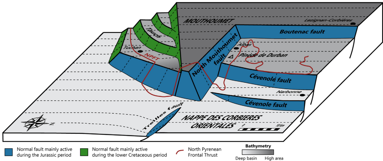
Fig. 10. 3D block showing the paleogeography of the study area during Mesozoic times. The current NCO front is shown in red. The faults, blue and green, highlight their main periods of activity: Jurassic and Albian-Cenomanian respectively.
