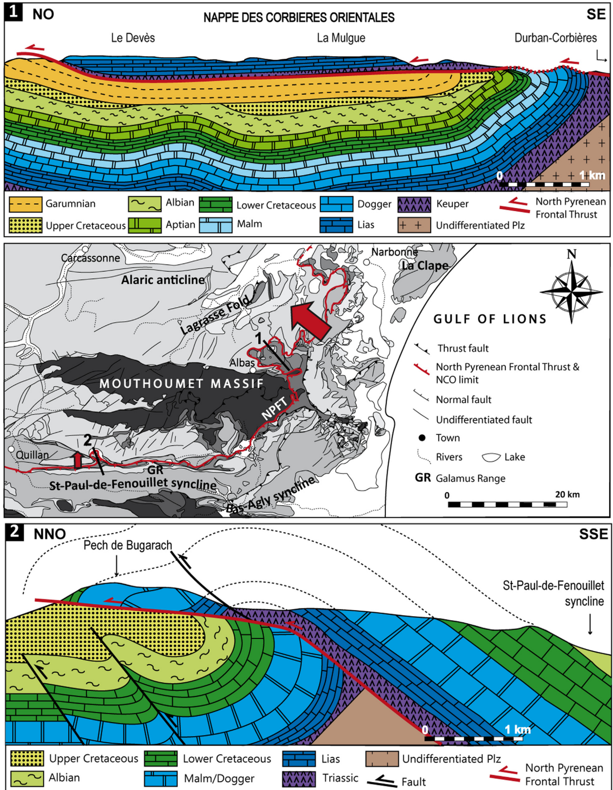
Fig. 11. Geological sections through the NCO (1) and the Bugarach ramp-anticline (see Fig. 1 for the location) (2) showing the shortening variation between the two structures. Refer to the Figure 1 for formations ages.
