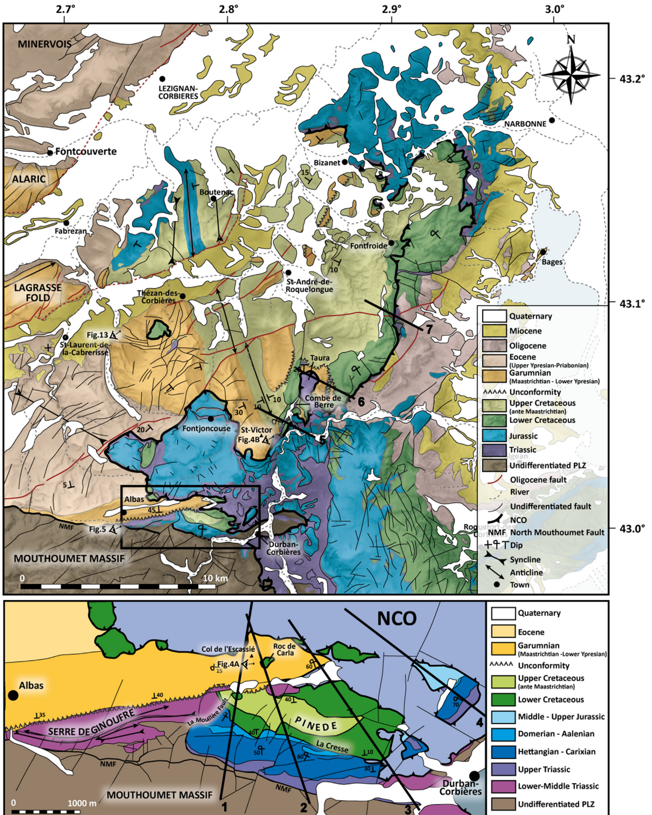
Fig. 3. Structural map of the NCO modified after Lézignan-Corbières, Béziers, Capendu, Narbonne, Tuchan and Leucate 1/50 000 BRGM geological maps (Ellenberger et al., 1987; Lespinasse, 1982; Berger, 1982; Berger et al., 1982, 1990, 1997) and focus on the geological map of the “Serre de Ginoufre” and the “Pinède de Durban” modified from Durand-Delga and Charrière (2012). Mapped cross-sections correspond to the geological sections in Figure 7.
