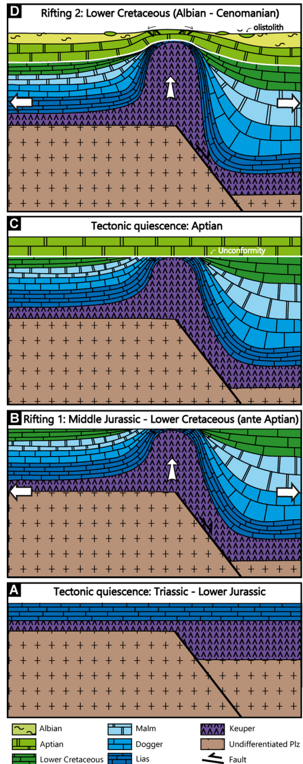
Fig. 9. Sketch illustrating the development of a salt diapir during the Mesozoic rifting episodes, from the Lower Jurassic to the Lower Cretaceous. Demonstrating the detail of the halokinetic sequences with the formation of the two distinct sedimentary wedges (Middle Jurassic-Lower Cretaceous, and Albian-Cenomanian). See the text for more details.
