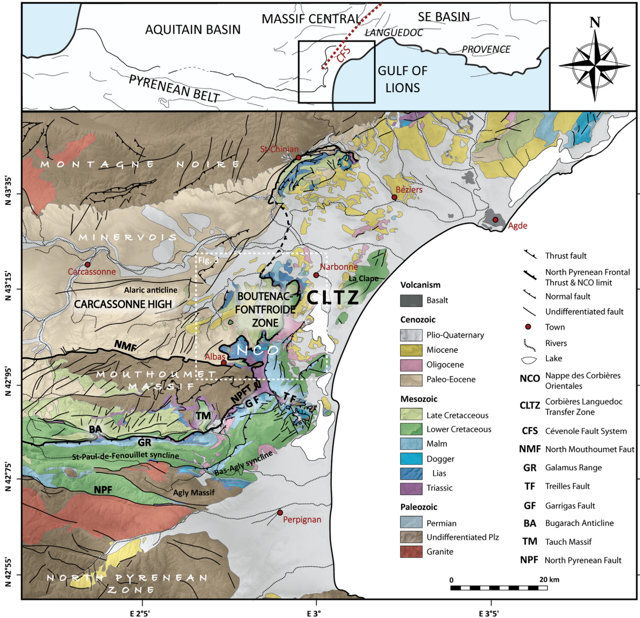
Fig. 1. Structural map of the Corbières area, Eastern Pyrenees. Modified after 1/50 000 and 1/80 000 BRGM geological maps.
