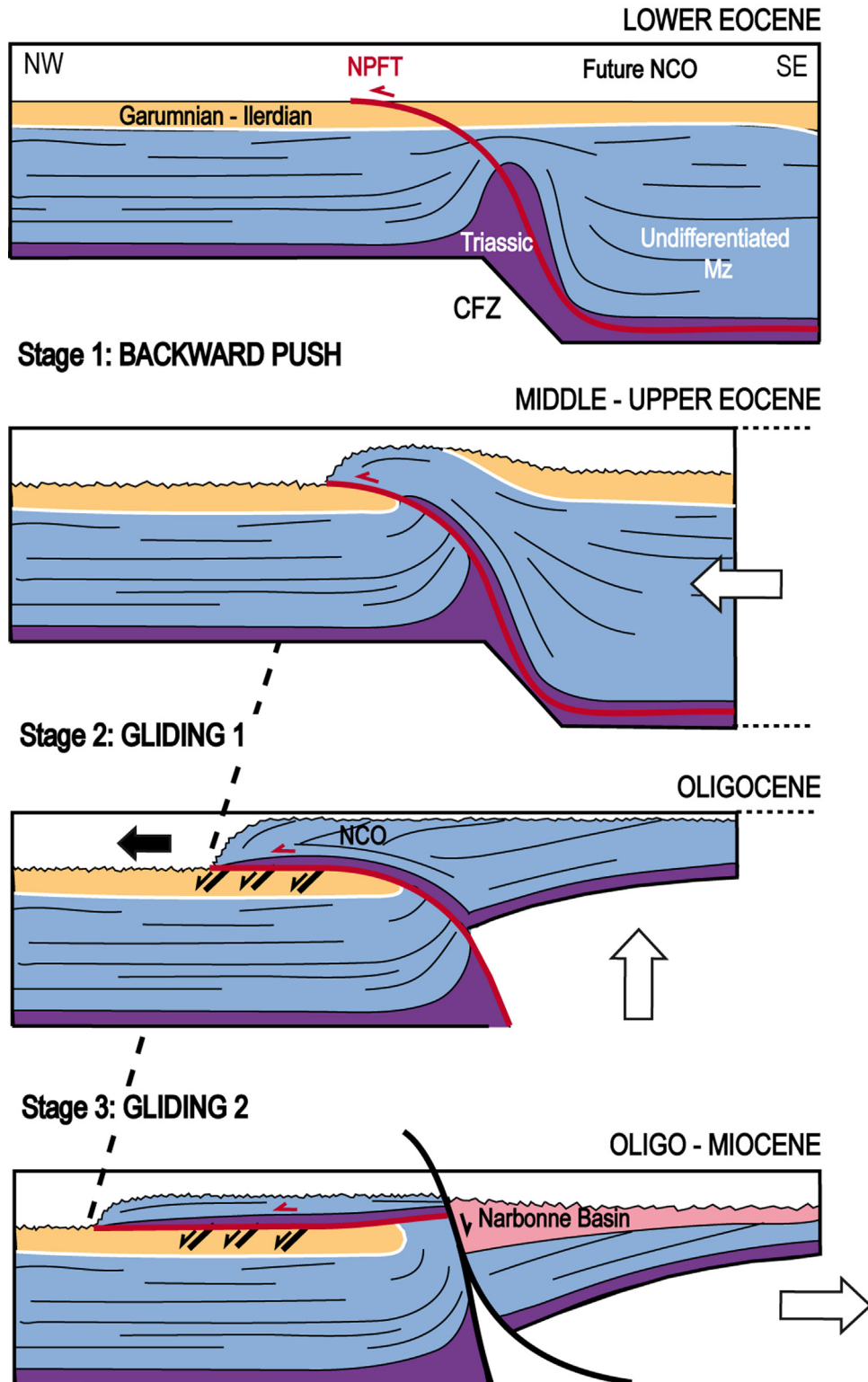
Fig. 12. Sketch illustrating the mechanisms of NCO emplacement from the Lower Eocene to the Oligo-Miocene. Stages 1 and 2: a thrust fault (prolongation of the NPFT) was developed during the Pyrenean orogeny along the Cévenole Fault System, thanks to a previously emplaced salt diapir. The thrust-fault has been then uplifted and flattened during two consecutive geodynamic episodes: an Oligocene uplift (stage 3) predating the Gulf of Lions rifting and the subsequent Miocene rifting (stage 4), creating a rift shoulder, west of the Narbonne basin.
