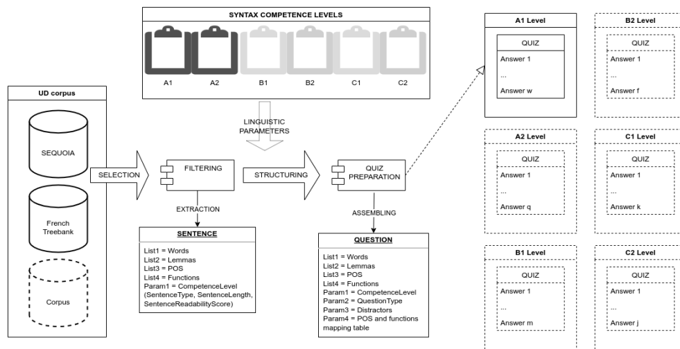
Figure 1: The corpus to quiz processing chain
