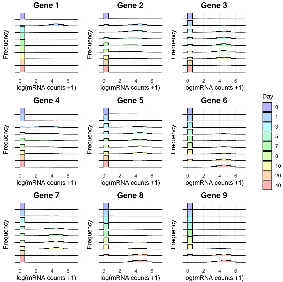
Figure 3: Time dependent evolution of mRNA distributions of 9 genes (see Figure 1A): x-axis shows the value of mRNA+1 in logarithmic scale, while y-axis shows the frequency observed at different time points.
