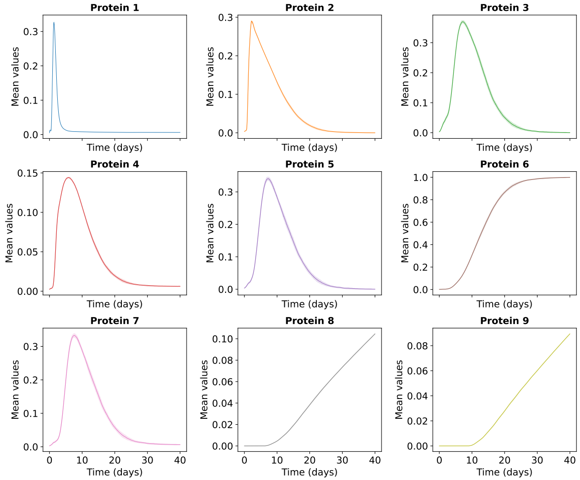
Figure 4: Time-dependent mean protein expressions over 10 simulations across all cells. Shown is the mean (solid line) \pm std (shaded area) for the 9 main genes of the augmented GRN.
