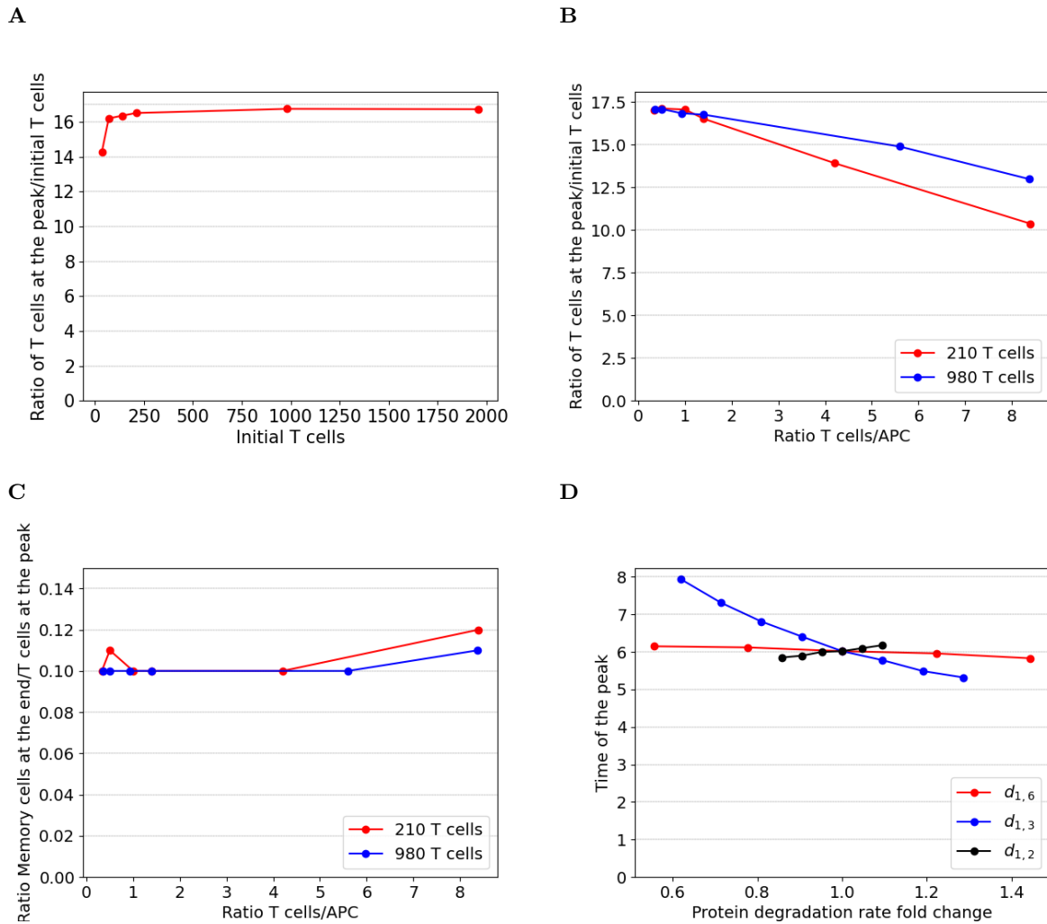
Figure 6: Comparison of variables of interest when varying initial cell counts. (A) Average cell expansion at the peak of the response as a function of initial cell numbers over 10 simulations. (B) Average cell expansion at the peak of the response as a function of the ratio of initial T cells to APCs counts, in two cases comprising 210 and 980 T cells. (C) Ratio of the average memory cell counts at the end of the simulation to average T cells count at the peak, as a function of the ratio of initial T cells to APCs counts, in two cases comprising 210 and 980 T cells. (D) Effect of proteins 2, 3 and 6 degradation rates upon the time of the peak (for a Ratio T cells/APC equals 1.4). Reference values of protein degradation rates are given in Table 3.
