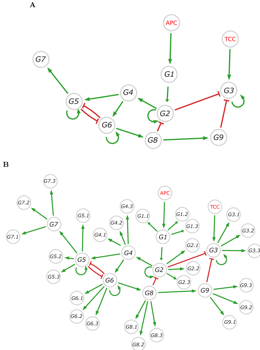
Figure 1: Schematic representation of the GRN. (A) The core circuitry of the principle-based GRN using 9 genes. The notation G_i corresponds to the gene number i . APC signalling and TCC signalling are perceived when CD8 T cells are in contact with APCs or effector cells, respectively. The green (resp. red) arrows represent activation (resp. inhibition). (B) The augmented GRN, made of 36 genes, incorporates the core principle-based GRN together with “decorating” genes. The gene G_{i,j} , j \in \{1, 2, 3\} , is the j -th gene activated by gene i .
