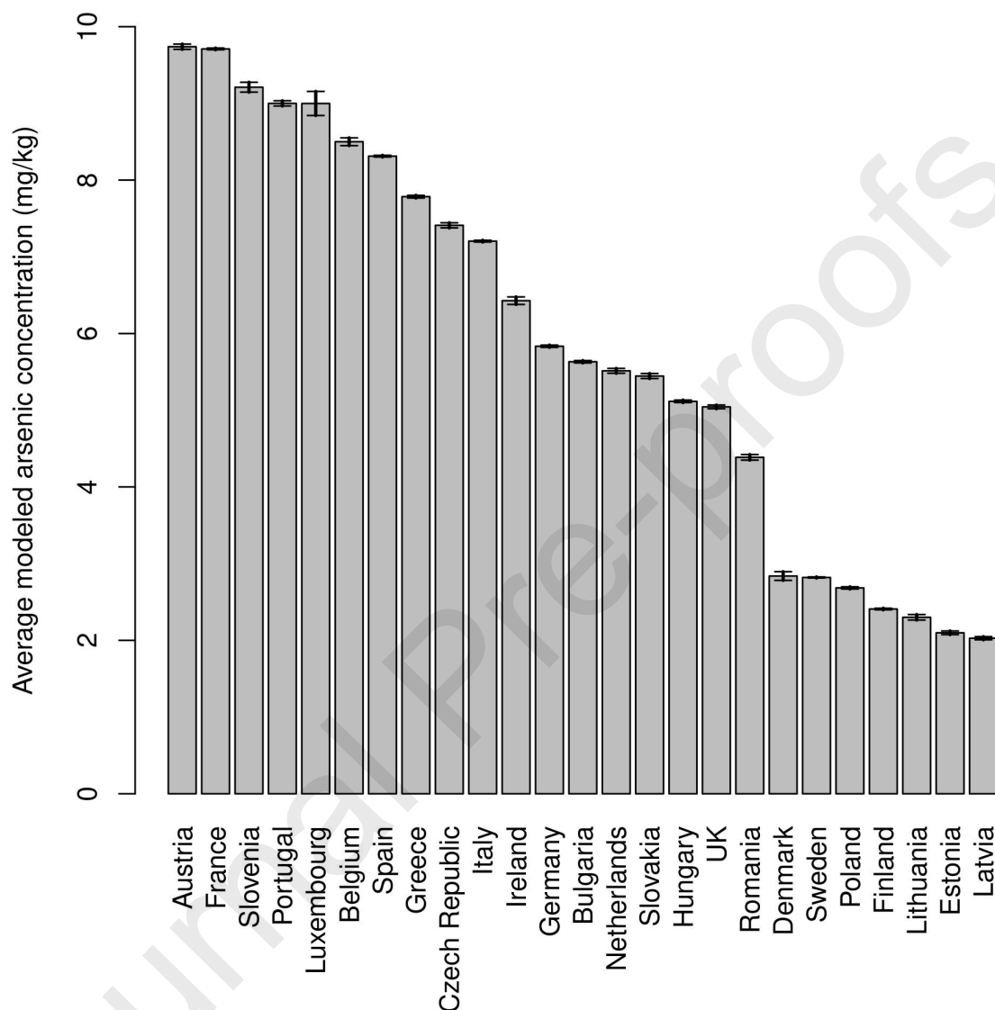
Figure 7 - Average modeled arsenic concentrations per European country. The uncertainty lines represent confidence intervals and are equal to two times the standard deviation of the 500 repetitions used to calculate the average.
