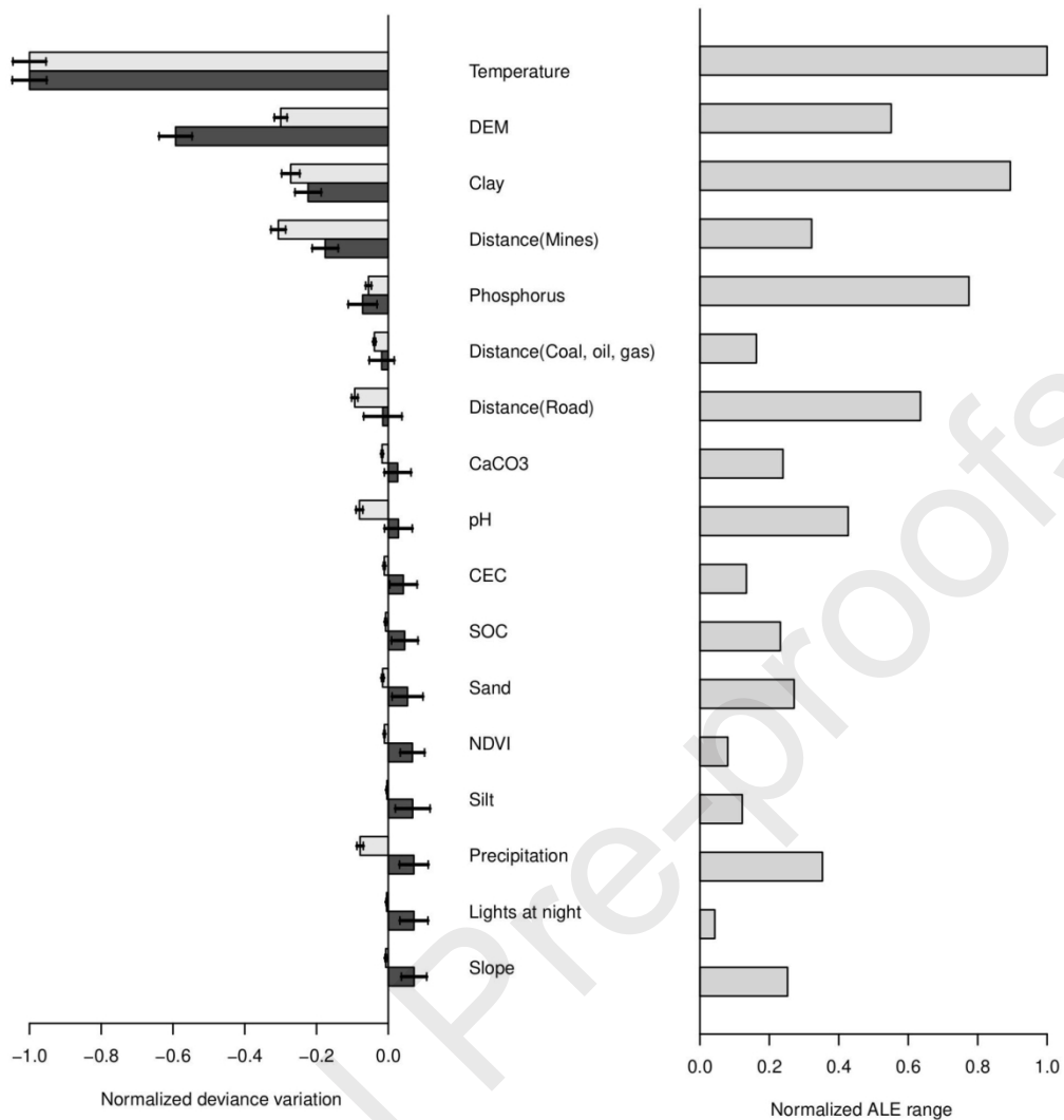
Figure 4 - Scaled importance measures: statistical measures based on the deviance variation (left) and a practical measure based on the Accumulated Local Effects (ALE) range (right). In the left plot, the feature permutation measure is shown in light gray and the leave-one-out measure, in dark gray. The uncertainty bars refer to the standard deviation of 250 repetitions of the method.
