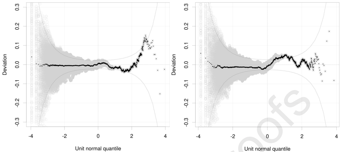
Figure 3 - Worm plot of the normalized randomized quantile residuals for the training dataset (left) and the validation dataset (right).
