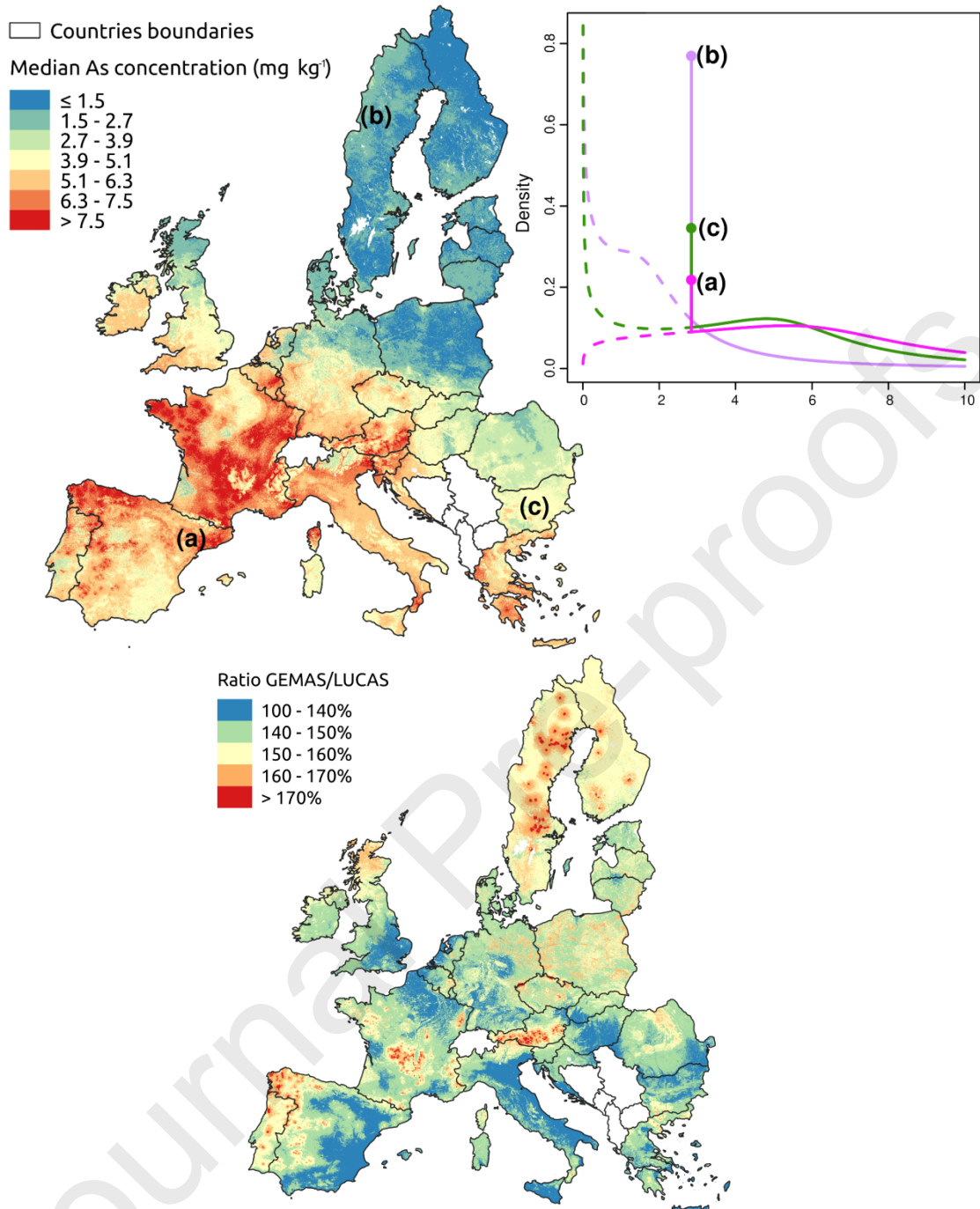
Figure 6 - Median arsenic concentrations in Europe: model predictions, along with three example points (top), and ratio between results using the GEMAS and the LUCAS database (bottom). In the top right plot, the continuous line is the probability density function for the censored logSHASHo distribution, while the dashed line shows the reconstructed left tail. The points on the vertical line show the corresponding fitted probabilities of being below the censor value 2.84 mg kg -1 . The bottom plot shows the ratio of predictions by the calibrated GEMAS model over the fitted LUCAS model.
