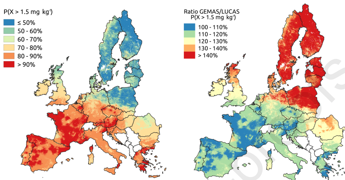
Figure 9 - Exceedance probabilities for the background concentration of 1.5 mg kg -1 . Results are predictions from the fitted LUCAS model (left), and the ratio of predictions with the calibrated GEMAS model (right).
