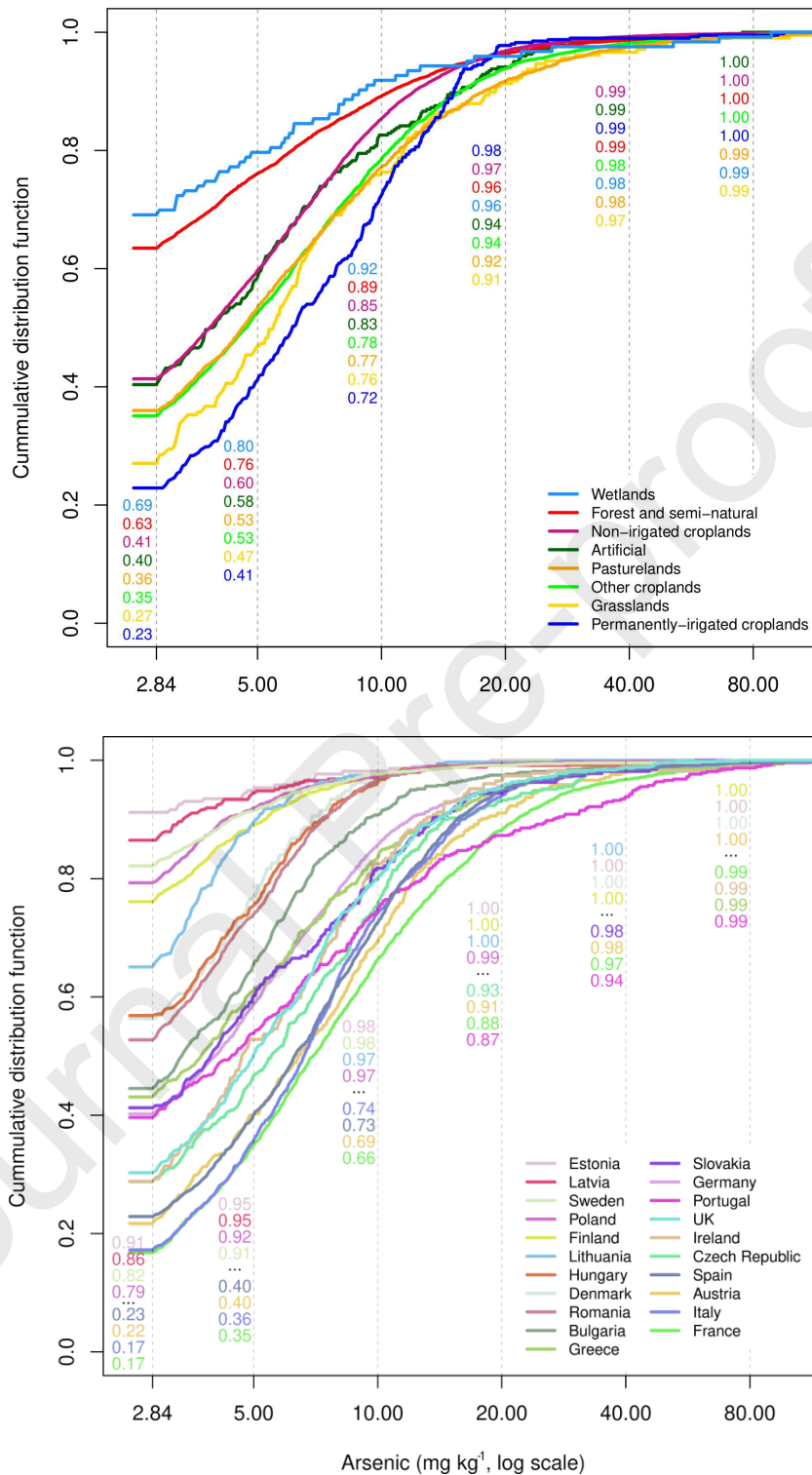
Figure 1 - Sample cumulative distribution of Arsenic stratified per land use (top) or country (bottom). The numbers in the top plot correspond to each land use class, while in the bottom plot correspond to the 4 top and bottom country classes.
