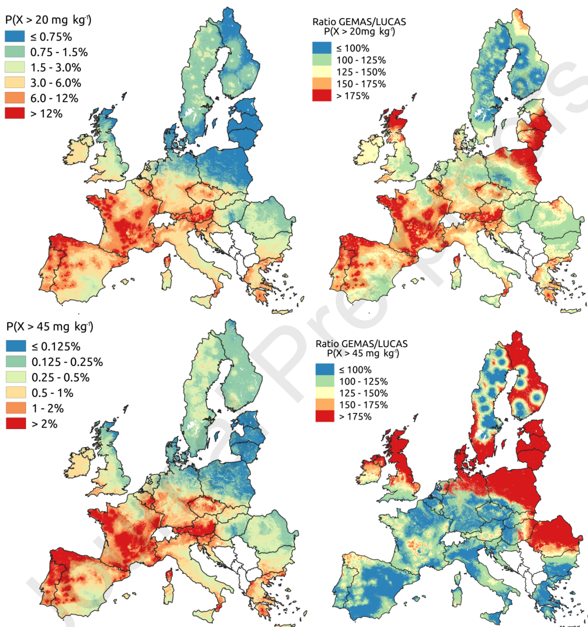
Figure 8 - Exceedance probabilities for two limits of action in Europe: 20 mg kg -1 (top) and 45 mg kg -1 (bottom). Results are predictions from the fitted LUCAS model (left), and the ratio of predictions from the calibrated GEMAS model to those of the LUCAS model (right).
