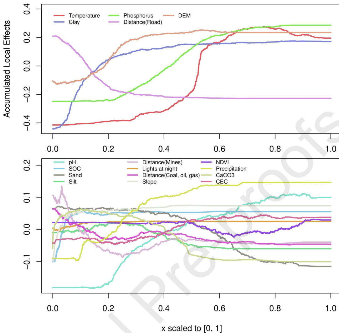
Figure 5 - Accumulated Local Effects (ALE) on the \mu parameter (i.e. the log of the median As concentration) for the 5 explanatory variables of higher practical importance (top) and the other variables (bottom). The distance variables are displayed in their original scale, not log-transformed.
