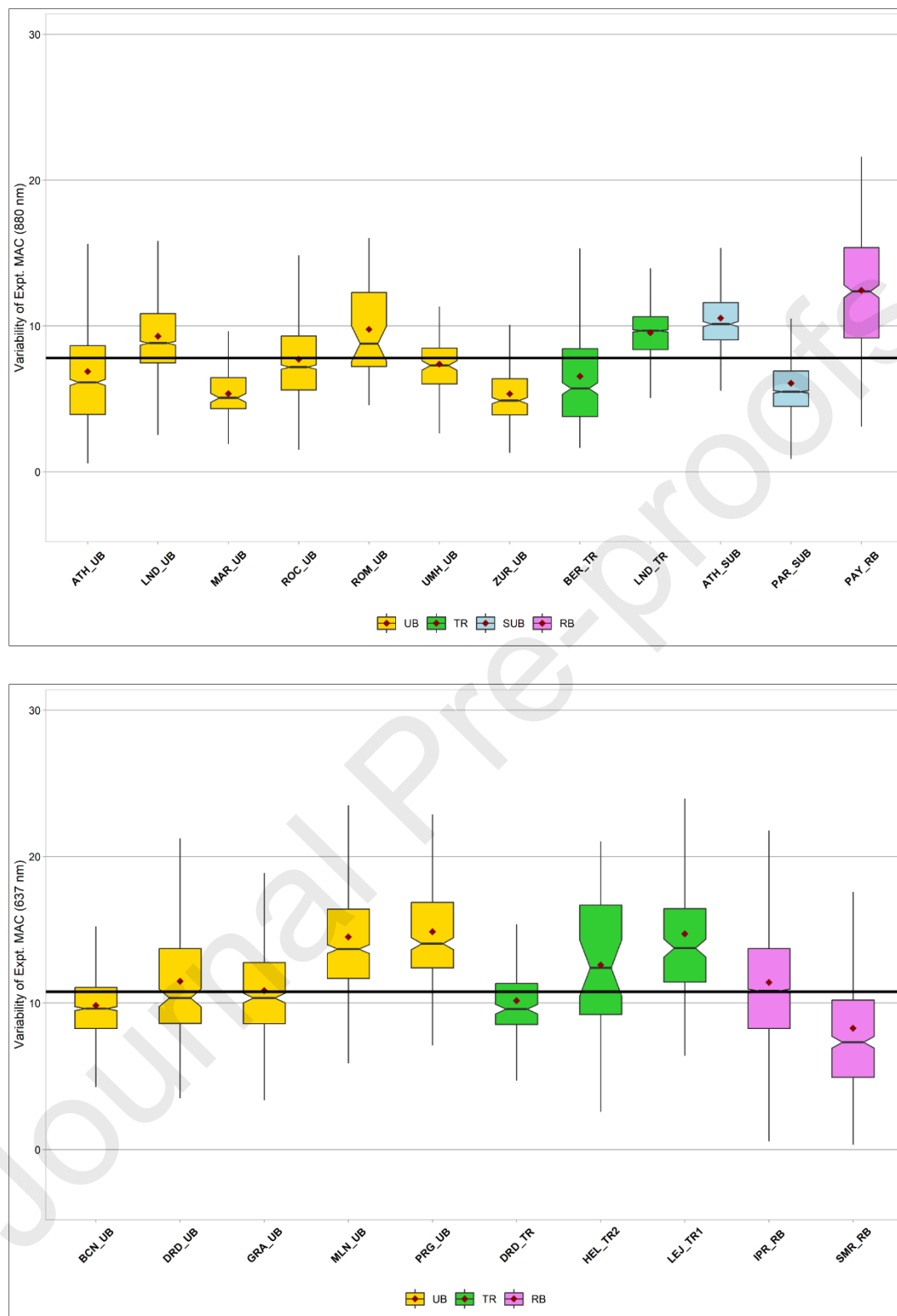
Figure 3. Variability in experimental MAC at instrument-specific wavelengths (MAAP: 637 nm; AEs: 880 nm) across 22 sites categorized by site type (UB, urban background; SUB, suburban background; TR, traffic; RB, regional background). The upper panel correspond to AEs at 880 nm, while the lower panel correspond to MAAP instruments at 637 nm. The solid black line represents the total experimental median MAC for 12 AEs at 880 nm ( 7.8 \pm 3.4 \text{ m}^2 \text{ g}^{-1} ) and 10 MAAPs at 637 nm ( 10.6 \pm 4.7 \text{ m}^2 \text{ g}^{-1} ). Box-and-whisker plots depict the 25th and 75th quartiles, with the median indicated by a notched inner line. The mean is represented by the red points within the box plots.
