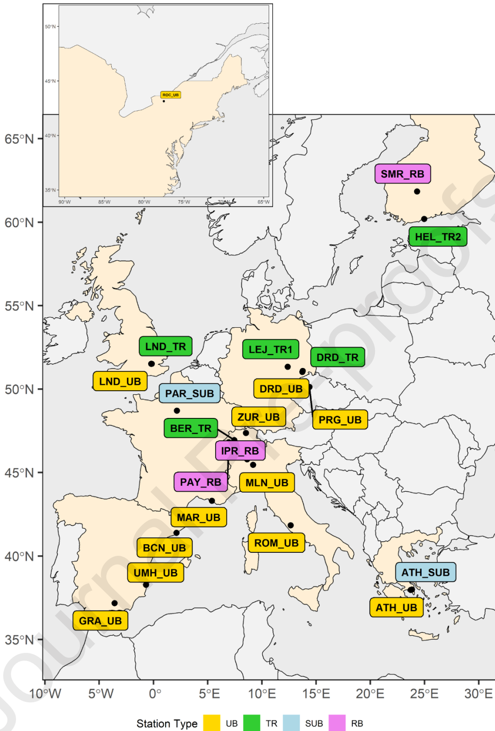
Figure 1. Location of the cities and type of 22 monitoring sites with eBC and EC mass concentration measurement data being supplied to this study, UB, urban background; SUB, suburban background; TR, traffic; RB, regional background.
