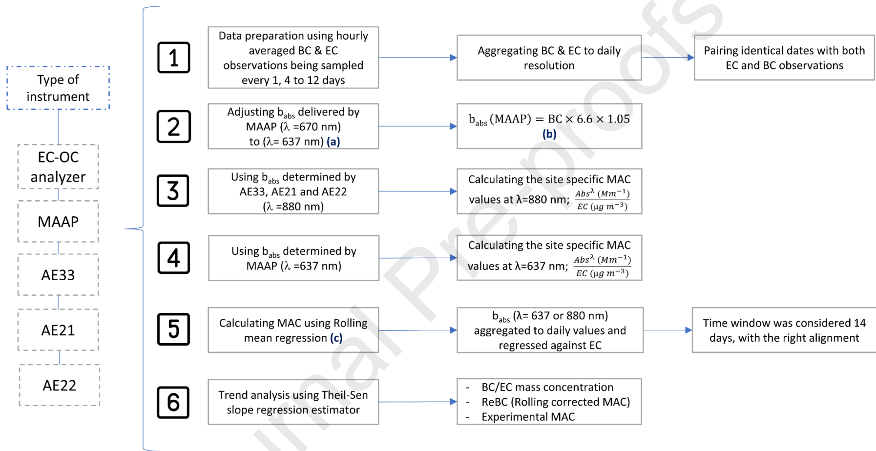
Figure 2. The overall scheme by which to process corrected and normalized eBC mass concentrations in order to obtain site-specific MAC values. More details are provided in sections 2.4, 2.5 and 2.6. (a): 637 nm is the reference wavelength of the MAAP to derive MAAP- equivalent absorption coefficient; (b): 1.05 is the correction factor to the true wavelength (637 nm); (c) Efficient Rolling/ Windowed Operations using “zoo” and “RcppRoll” R packages.
