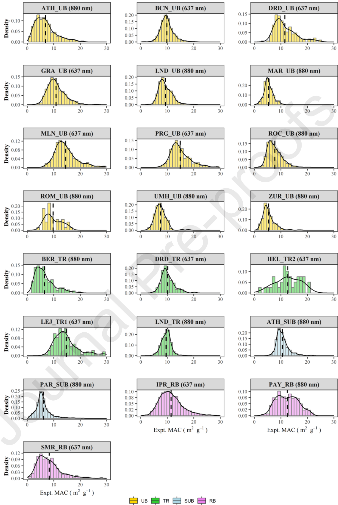
Figure 4. Frequency distribution of experimental MAC for the whole available period. The color shading represents the type of site (UB, urban background; SUB, suburban background; TR, traffic; RB, regional background). The corresponding median MAC is shown in black sticks.
