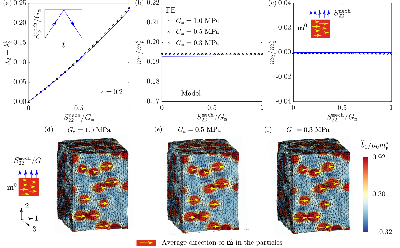
Figure 13: Evolutions of (a) mechanical stretch \lambda_2 - \lambda_2^0 (with \lambda_2^0 denoting the initial remanent stretch due to the pre-magnetization) and magnetizations along (b) \mathbf{e}_1 and (c) \mathbf{e}_2 under applied uniaxial tensile stress S_{22}^{\text{mech}} , whose temporal evolution is shown in the inset of (a). The inset of (c) shows a schematic of the h -MRE with the direction of pre-magnetization \mathbf{m}^0 and the applied uniaxial tension. Contours of the \tilde{\mathbf{b}} field in the deformed RVE under applied S_{22}^{\text{mech}}/G_m = 1 for G_m = (d) 1.0, (e) 0.5 and (f) 0.3 MPa. The arrows on the particles show the average direction of \tilde{\mathbf{m}} in them. (Taken from Mukherjee et al. (2021)).
