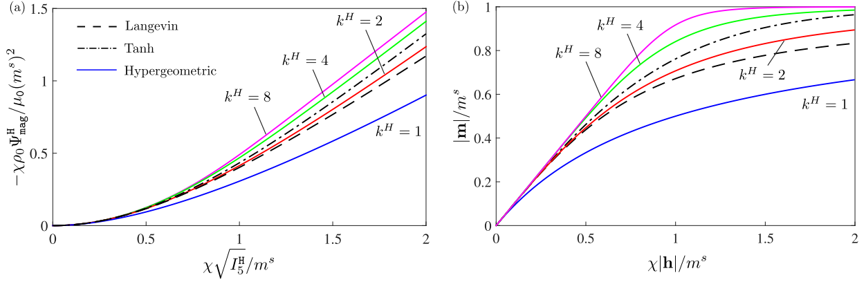
Figure 4: Comparison of (a) the magnetic energy functions and of (b) their derivatives obtained from and hypergeometric \Psi_{\text{mag}}^H saturation function given in equation (82) for various exponents k^H , the Langevin function and the hyperbolic tangent function (see (85)). (Taken from Mukherjee et al. (2020)).
