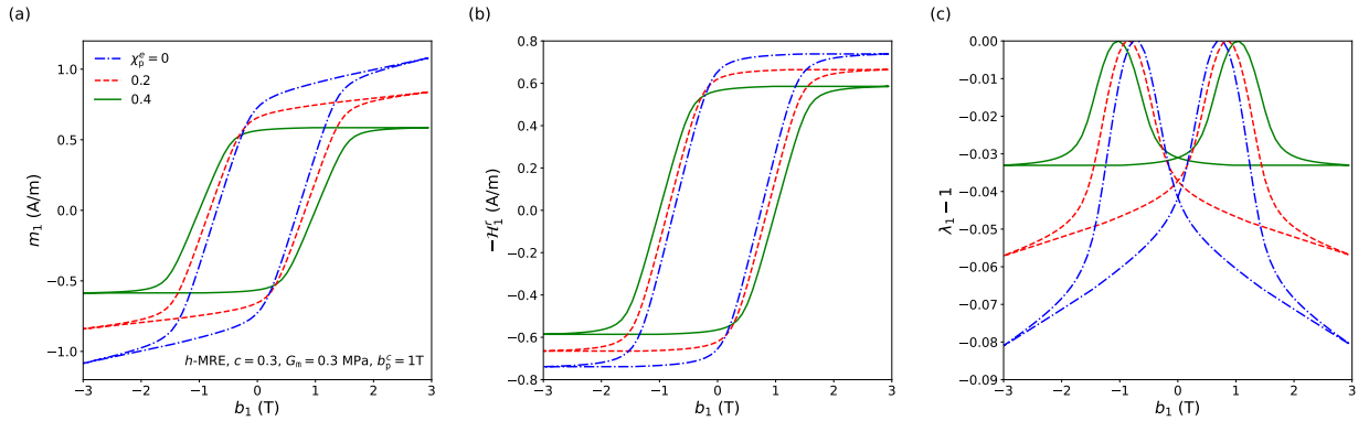
Figure 11: Comparison of the (a) magnetization m_1 , (b) (minus) internal variable -\mathcal{H}_1^T and (c) magnetostriction response \lambda_1 - 1 as predicted by the h -MRE model for three values of \chi_p^e = 0, 0.2, 0.4 , coercivity b_p^c = 1 T, particle volume fraction c = 0.3 and matrix shear modulus G_m = 0.3 MPa.
