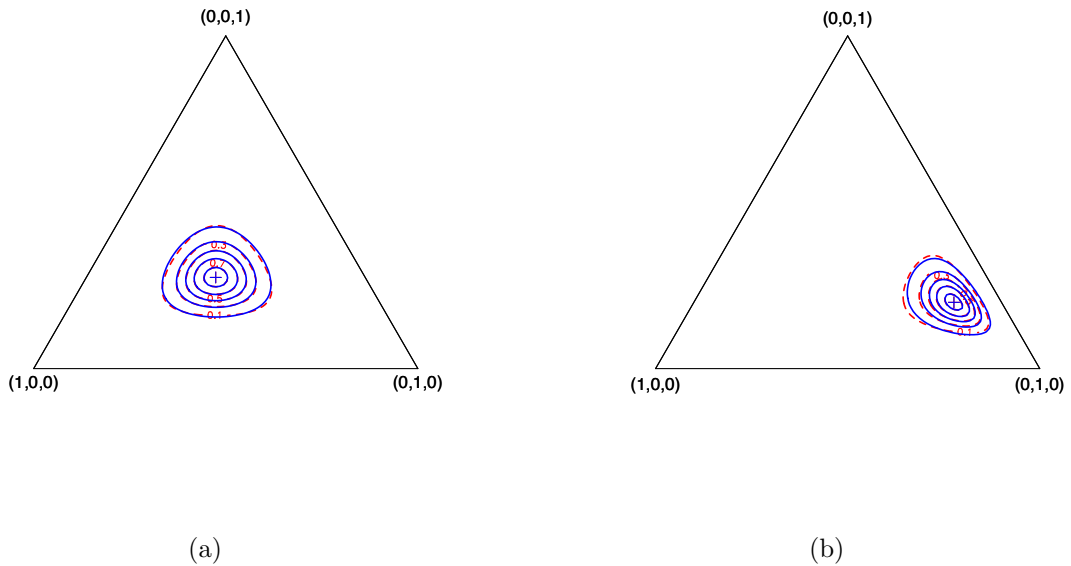
Figure 7: Contours at levels 0.1, 0.3, 0.5, 0.7 and 0.9 of possibility distributions \pi_{\theta(x)|\mathbf{y}} for x = (0.1, -0.5) (a) and x = (-0.35, -0.47) (b) for the Wine dataset (blues solid lines), and normal approximations (red broken lines).
