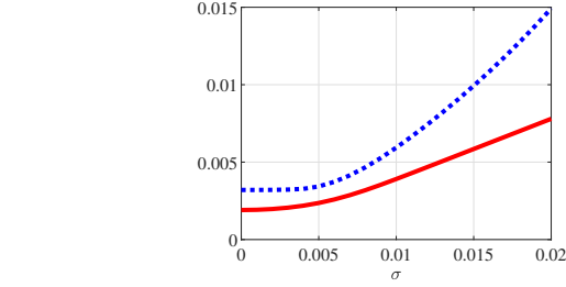
Figure 3. Illustration of the noise propagation factor (in red/solid) and its upper bound in Corollary III.4 (in blue/dotted) for the Gaussian PSF per varying \sigma ( N = 501 , \Delta = 0.25 , N\Delta \approx 125 ).
