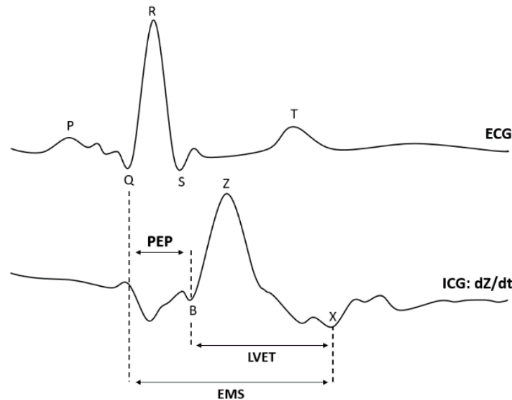
Figure 1: ECG and ICG signals are represented by different main waves and the PEP, LVET, and EMS intervals. ECG: electrocardiogram; ICG: impedance cardiography; PEP: pre-ejection period; LVET: left ventricular ejection time; EMS: electro-mechanical systole.
