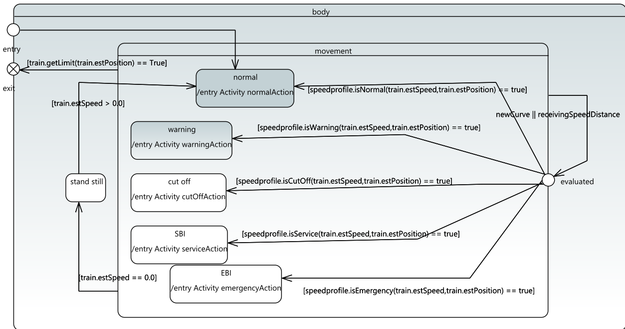
Fig. 6.65. Supervision sub-SMD
