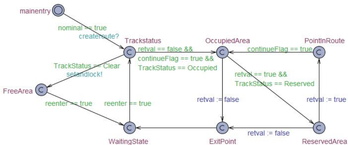
Fig. 8.14. CreateRoute automaton
