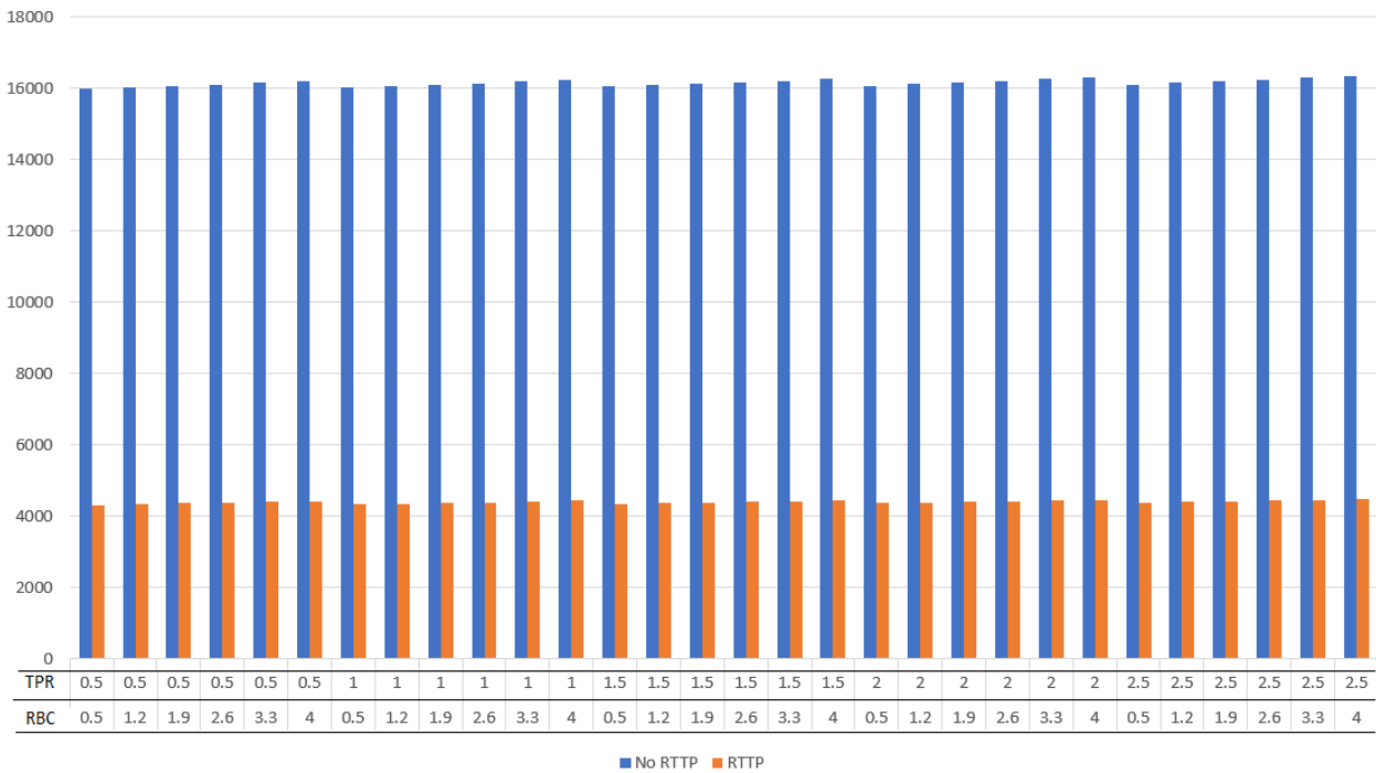
Figure 13: Scenario 4 (20 min delays) total lateness with and without traffic management (RTTP).
