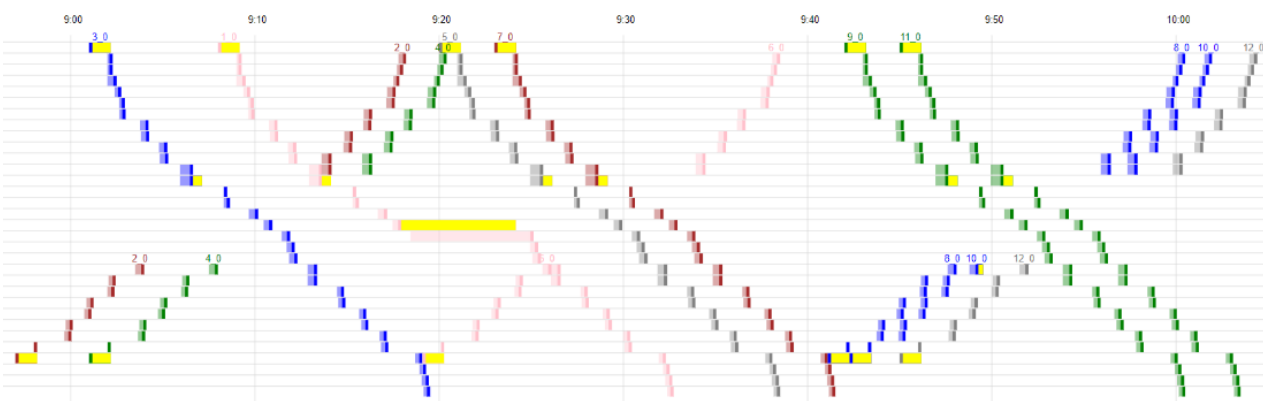
Figure 16 Blocking time diagram of optimised traffic plan for scenario 2.
