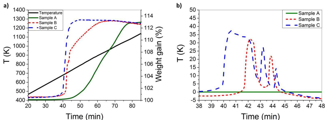
Figure 5 a) Mass gain profile for samples A, B and C vs. temperature and time; b) Sample holder temperature increase during ignition of samples B and C.
