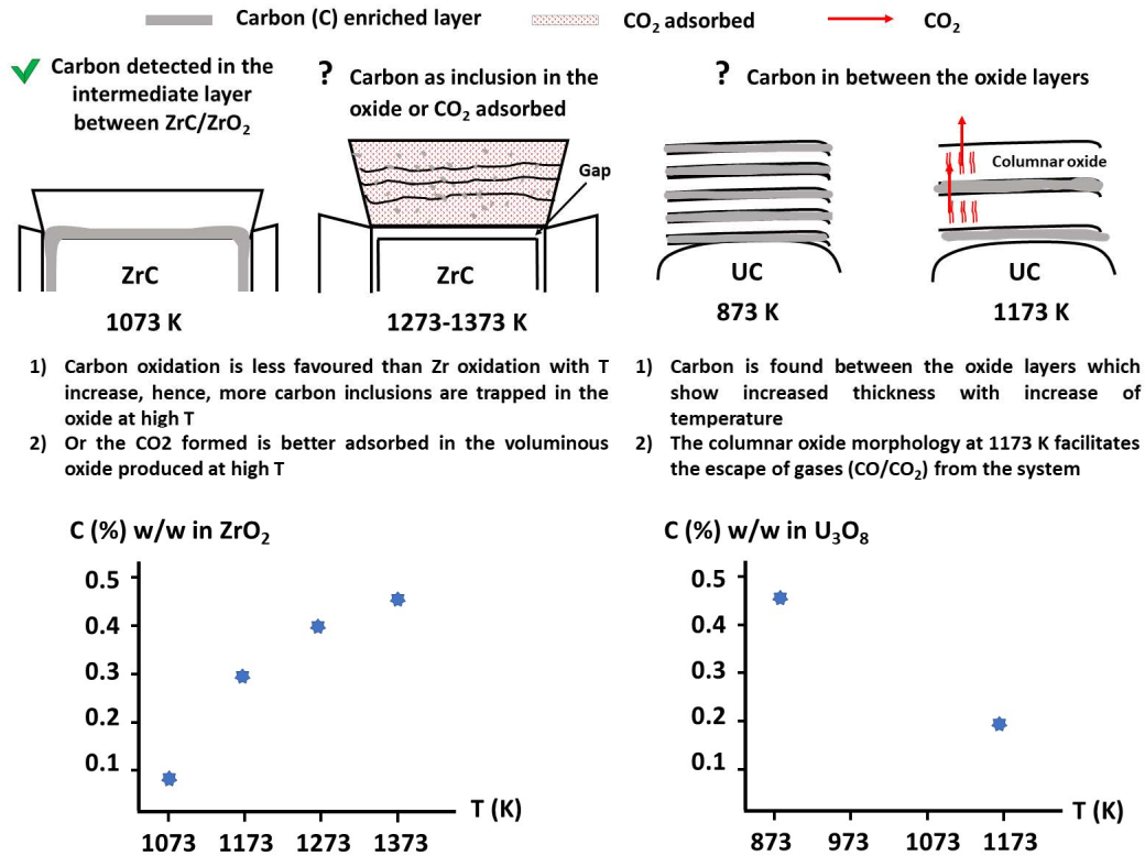
Figure 10 Schematic that shows the fate of carbon or CO 2 in the oxide formed from oxidation of ZrC and UC in air (amorphous carbon was characterised in the intermediate layer between ZrC/ZrO 2 [29] in samples oxidised at 1073 K with transmission electron microscopy). Note the opposite trend between carbon concentration and temperature in oxide formed in UC or ZrC oxidations.
