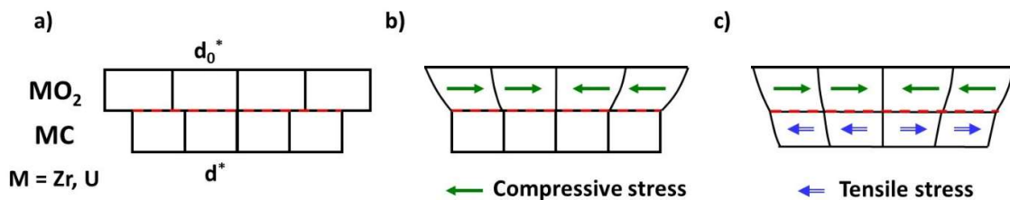
Figure 11 Schematic of the system considered for approximate strain and stress analysis, the effect of the intermediate layer between carbide and oxide (highlighted with a dashed red line) was not considered: a) ideal system where the oxide layer does not show any epitaxial relations to the carbide, b) system used for strain and stress calculations: the oxide layer is constrained to assume the structure of the carbide layer, c) both the carbide and oxide layers show stresses induced by epitaxial growth (this is closer to reality but difficult to obtain information from)
