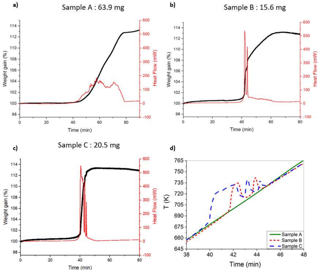
Figure 4 TGA/DSC signals during UC oxidation from 298 - 1673 K in air a) gradual oxidation (Sample A), b) ignition (Sample B), c) rapid ignition (Sample C), d) sample holder temperature profile of samples A, B and C: crucible overheated due to self-ignition mechanism in Sample B and C.
