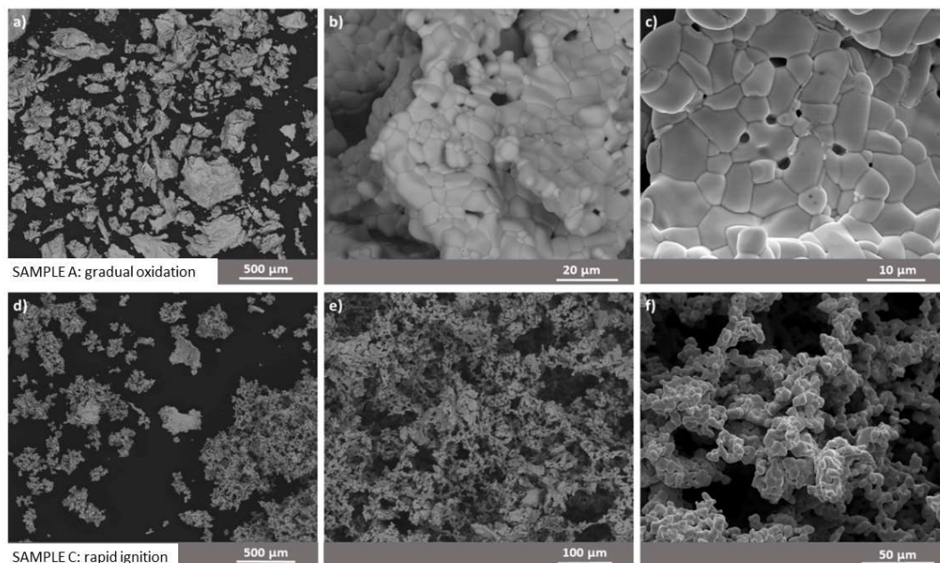
Figure 6 BSEI (a, b, d and e) and SEI (c and f) of sample A (top row) and sample C (bottom row).
