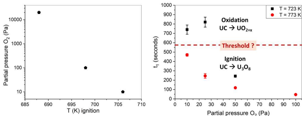
Figure 7 a) Temperature at which UC ignition was triggered on fragments exposed to a thermal ramp mode at various oxygen partial pressure, b) Time constants t_1 (seconds) evaluated on area % plotted against oxygen partial pressure of UC samples oxidised at 723 K and 773 K in isothermal mode [23]: above the threshold UC ignition was not triggered, samples simply oxidised
