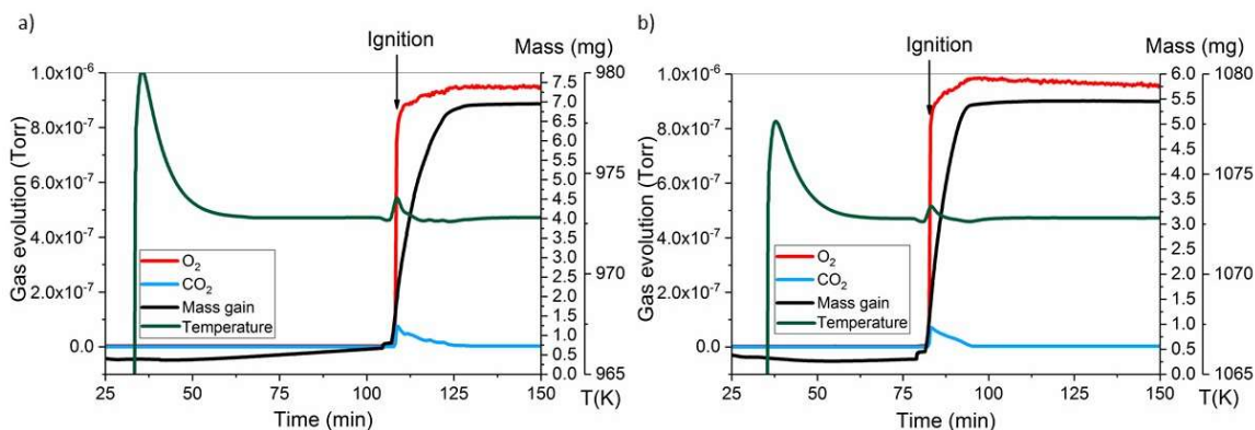
Figure 8 TGA/DTA-MS data for fragments chosen from air-stored UC pellet oxidised in air at 973 (a) and 1073 K (b). The sharp temperature increase and steep mass increase are characteristics of ignition
