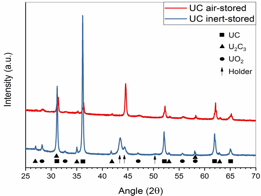
Figure 2 XRD characterisation of UC fragments which were crushed and kept in air atmosphere (air-stored) or in inert atmosphere (inert-stored), from Dounreay legacy fuels. Peaks were identified against PDF 01 073 1709[36] for UC, PDF 01 074 0805[37] for U_2C_3 , and PDF 00 041 1422 for UO_2 [38]
