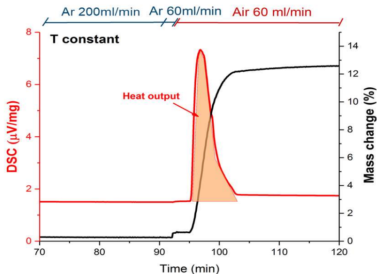
Figure 3 TGA/DTA run performed on air-stored and inert-stored fragments, this is a representative curve since both experimental conditions showed the same profile. The area highlighted under the DTA peak represents the heat output evaluated in \mu\text{V}/\text{mg} .
