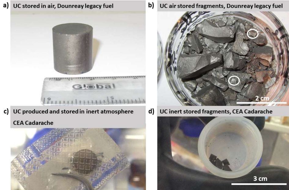
Figure 1 Photographs of a) Dounreay legacy fuel pellets and b) type of fragments chosen to be tested in TGA experiments; c) CEA Cadarache pellet and d) type of fragments chosen to be tested in HT-ESEM
