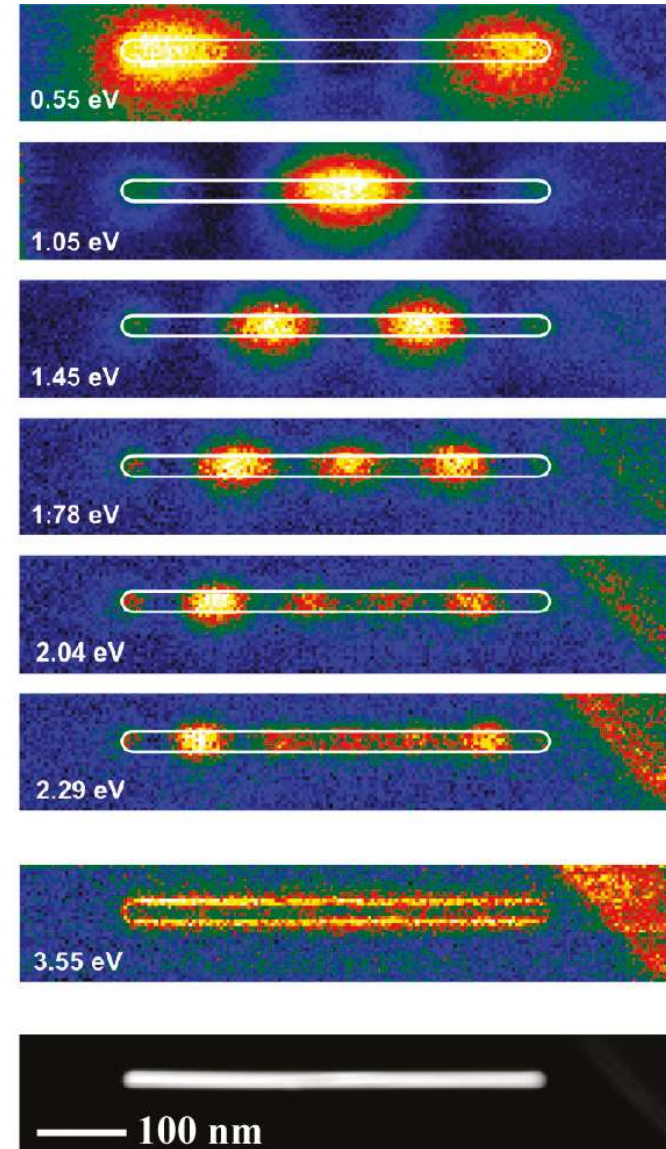
Ag NanoRods, 14 nm in diameter
