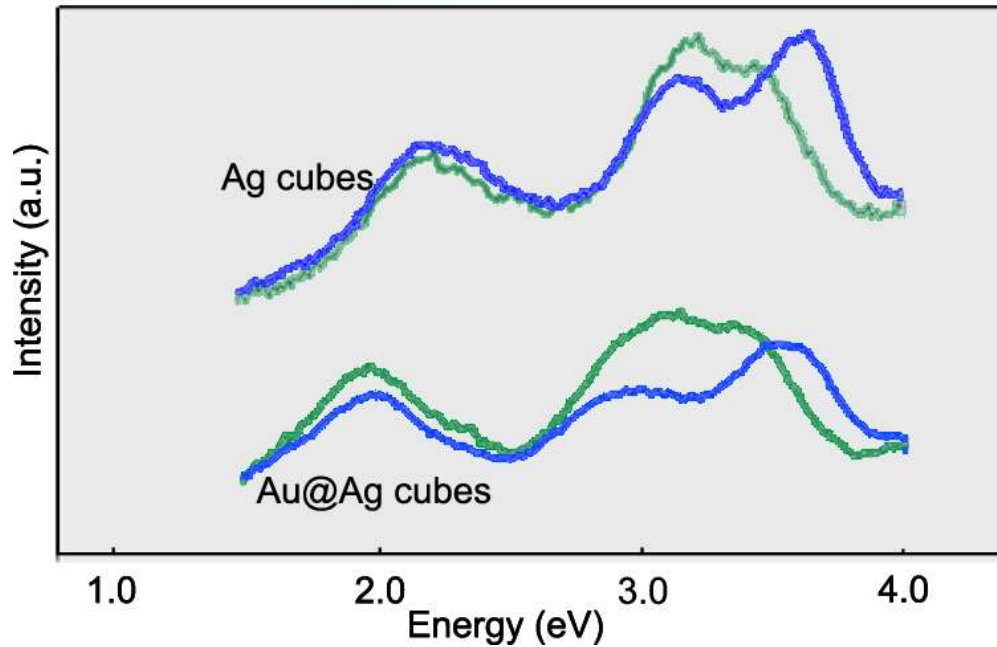
Ag and Au@Ag NanoCubes 70 nm
