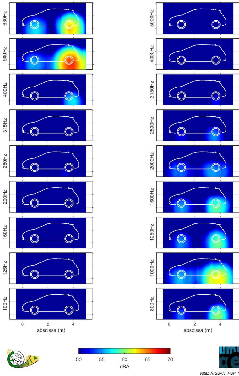
Figure F.2: Third-octave noise source maps of the Nissan LEAF#2 at constant speed 49.4 km/h on test section P – A-weighted noise levels at the reference distance 2.7 m – Colour scale in 0.5 dB(A) steps.
