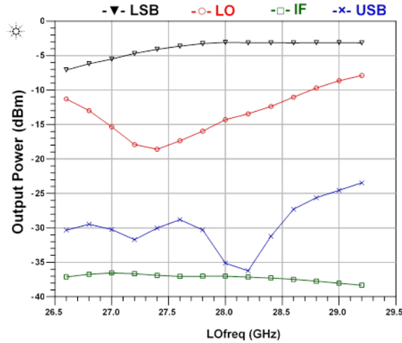
Figure 4. Variation of IF, LO, USB and LSB power versus LO frequency (for IF_power=-11.5 dBm and LO_power=7.5 dBm and IF_freq=2 GHz)
