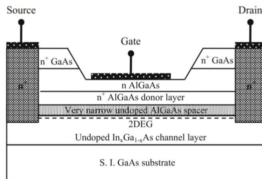
Figure 1. Structure of the pHEMT Technology [26]
