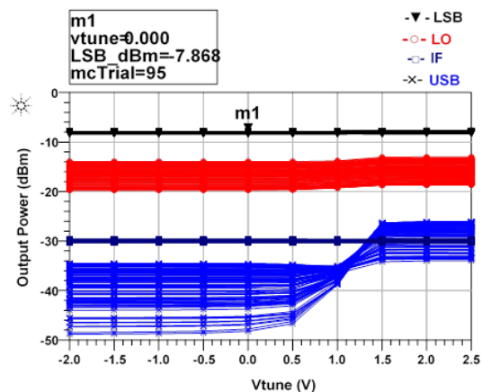
Figure 12. Monte Carlo analysis of IF, LO, USB and LSB power (for IF_power=-11.5 dBm and IFfreq=2 GHz)
