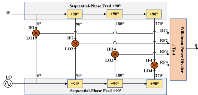
Figure 2. Synoptic diagram of the proposed double balanced mixer
