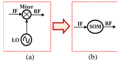
Figure 7. LO and Mixer blocks (a) before integration and (b) after integration
