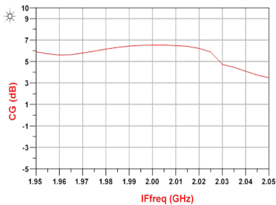
Figure 5. Variation of the conversion gain versus IF frequency (for IF_power=-11.5 dBm and LO_power=7.5 dBm and LO_freq=27 GHz)
