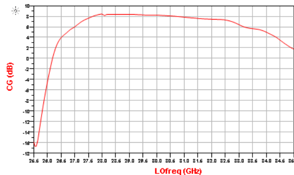
Figure 3. Variation of the conversion gain versus LO frequency (for IF_power=-11.5 dBm and LO_power=7.5 dBm and IF_freq=2 GHz)
