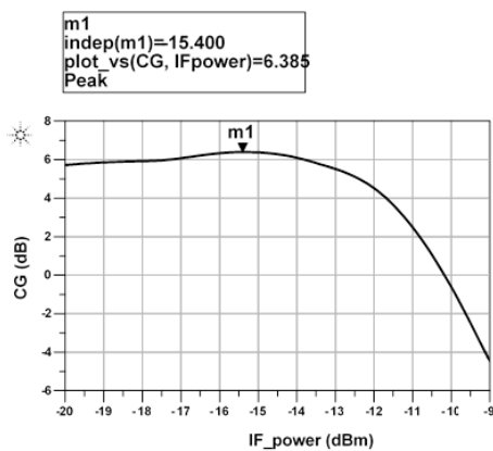
Figure 9. Variation of the conversion gain versus IF power (for IF_frequ=2 GHz, and LO_power=7.5 dBm and V_{tune}=0.8 V)
