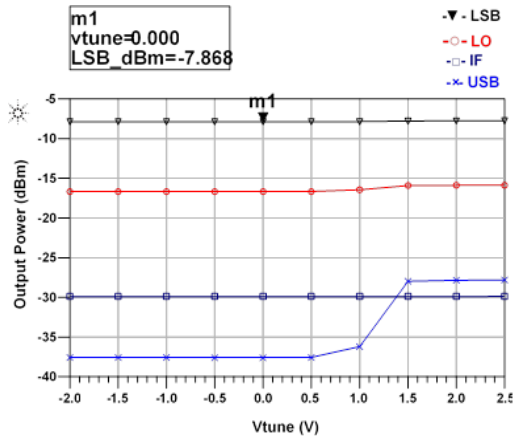
Figure 11. Variation of IF, LO, USB and LSB power versus vtune (for IF_power=-11.5 dBm and IFfreq=2 GHz)
