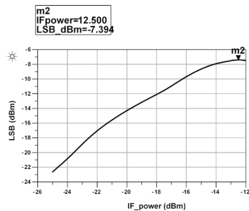
Figure 10. LSB power versus IF power (for IF_frequ=2 GHz, and LO_power=7.5 dBm and v_{tune}=0.8 V)
