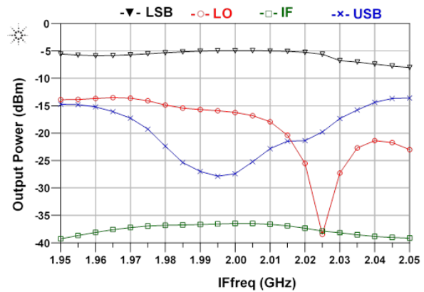
Figure 6. Variation of IF, LO, USB and LSB power versus IF frequency (for IF_power=-11.5 dBm and LO_power=7.5 dBm and LO_freq=27 GHz)
