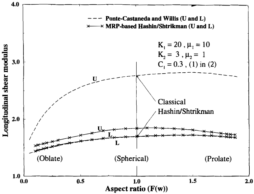
Fig. 11. Comparison between MRP-based and Ponte Castañeda and Willis upper (U) and lower (L) bounds. Composite with aligned ellipsoidal inclusions—longitudinal shear modulus \mu_{zz} .
