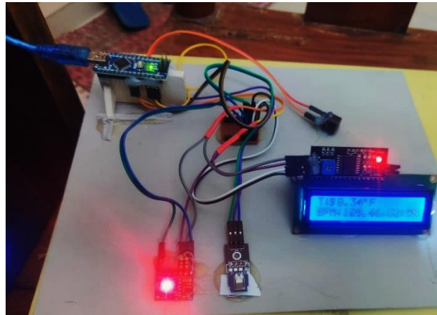
Fig. 12. Experimental result when user 2 pressed on the MAX30100 sensor
