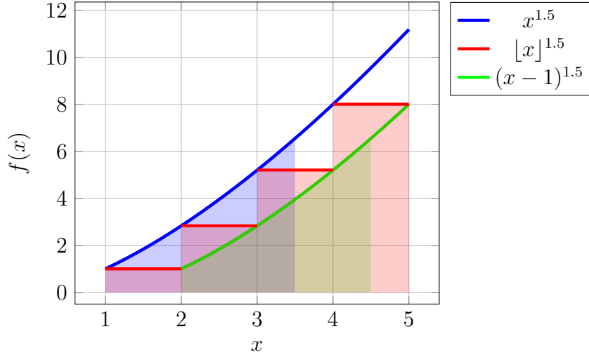
Figure 2: Illustration of the inequality \sum_{i=1}^{\lceil s \rceil} i^{-\alpha} \geq \int_1^s x^{-\alpha} dx for the case \alpha < 0 . In this example we have \alpha = -1.5 , s = 3.5 and \lceil s \rceil = 4 . The red area equals to the sum. The blue area equals to the integral and to the green area, which is fully under the red one.
