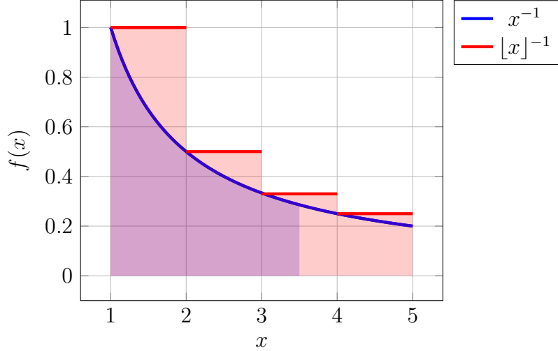
Figure 1: Illustration of the inequality \sum_{i=1}^{\lceil s \rceil} i^{-\alpha} \geq \int_1^s x^{-\alpha} dx for the case \alpha \geq 0 . In this example we have \alpha = 1 , s = 3.5 and \lceil s \rceil = 4 . The red area equals to the sum. The blue area (fully under red, thus purple) equals to the integral.
