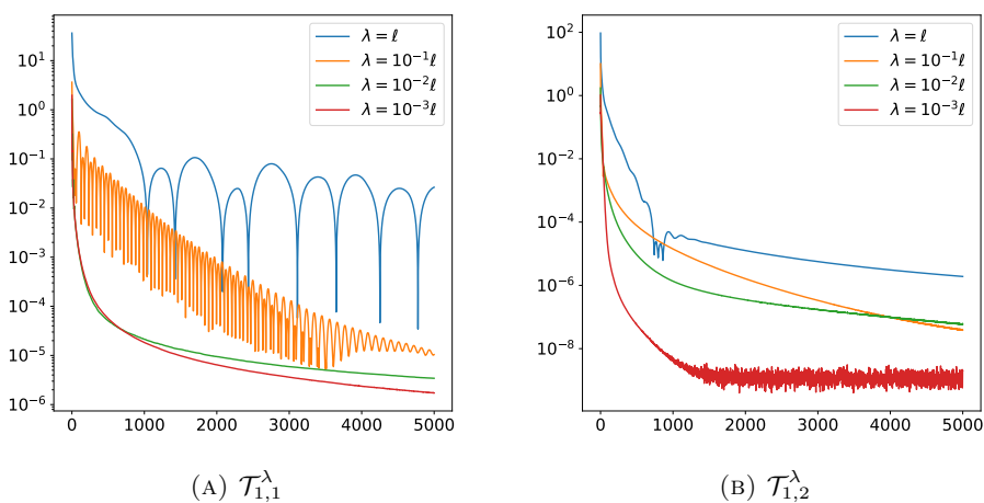
FIGURE 7. Convergence profiles of algorithm 1 for the error \Delta^n + r^n in Remark 4.5, for the different test cases of Section 5.4.
