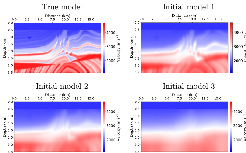
FIGURE 8. True velocity model of the Marmoussi test case and several initial conditions for the inversion problem.
