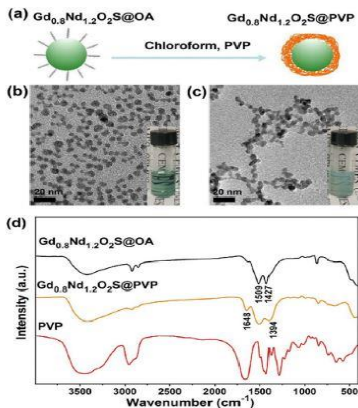
Fig. 3 Ligand exchange with PVP. (a) Schematic illustration of the synthesis of PVP-coated Gd_{0.8}Nd_{1.2}O_{2}S NPs. (b and c) TEM images of OA-coated and PVP-coated Gd_{0.8}Nd_{1.2}O_{2}S NPs. Inset photos show the dispersity of nanoparticles in cyclohexane and water with the same concentration of 10 \text{ mg mL}^{-1} , corresponding to before and after ligand exchange, respectively. (d) FTIR spectra of OA-coated, PVP-coated Gd_{0.8}Nd_{1.2}O_{2}S NPs and PVP.
