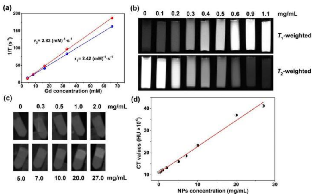
Fig. 5 MR and CT imaging. (a) T_1 and T_2 relaxivity plots of the aqueous suspension of PVP-coated Gd_{0.8}Nd_{1.2}O_2S NPs at 0.47 T. (b) T_1 - and T_2 -weighted MRI of PVP-coated Gd_{0.8}Nd_{1.2}O_2S NPs at 7 T for increasing concentration of NPs from 0 to 1.1 mg\ mL^{-1} . (c) CT imaging intensity variation with increasing concentration of PVP-coated Gd_{0.8}Nd_{1.2}O_2S NPs from 0 to 27 mg\ mL^{-1} . (d) Plot of HU as a function of NPs concentration.
