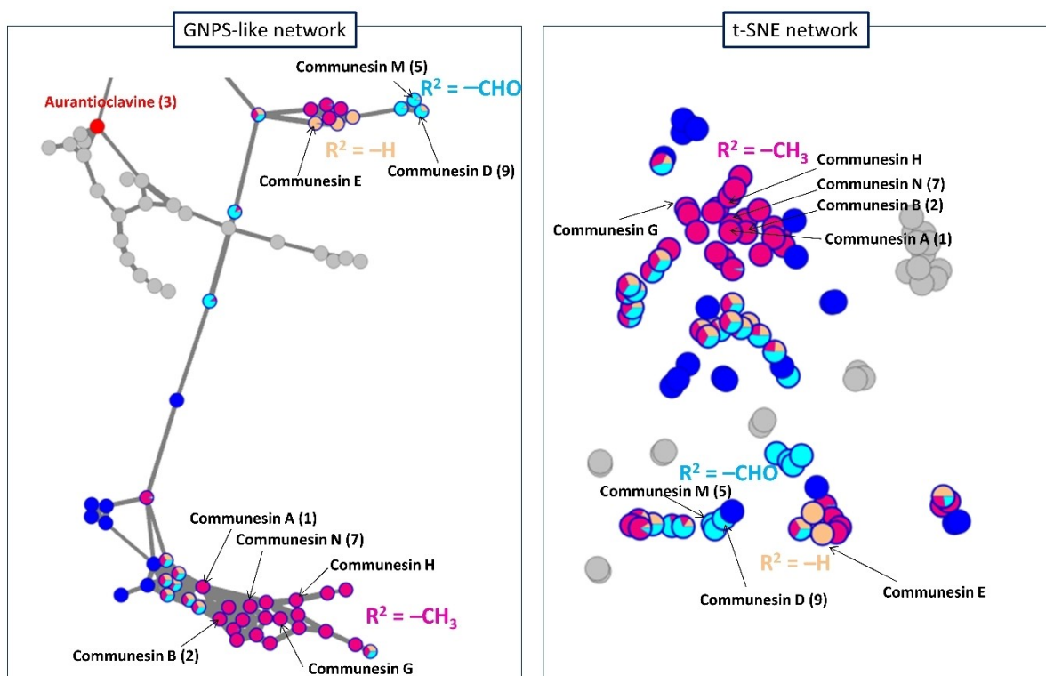
Figure 2. Determination of the most probable R^2 substituent based on the score calculated for each of the three possibilities: -H (orange), -CHO (bright blue) and -CH 3 (pink) and based on relative intensities of previously reported typical fragments observed for DME communesins. [4f] Blue nodes correspond to DME communesins with unidentified R^2 substituent. Known and new communesins detected in this study are highlighted.
