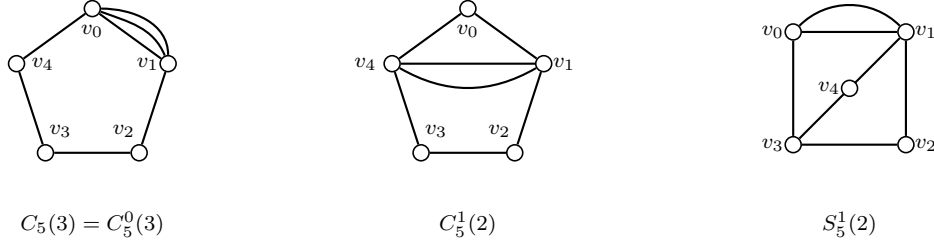
Figure 1: The graphs composing the set \tilde{\mathcal{S}}(7, 4) .
