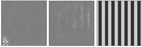
(a) Case with scorer targeting only the backdoored class
