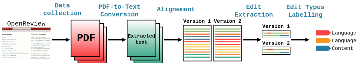
Figure 2: Steps of the creation process of the CASIMIR corpus
