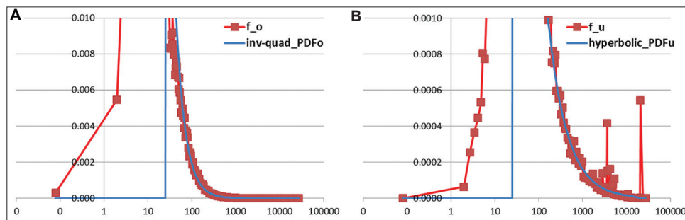
Figure 7. Approximations of (a) offered density PDF and (b) used density PDF Abscissas in log-scale.
