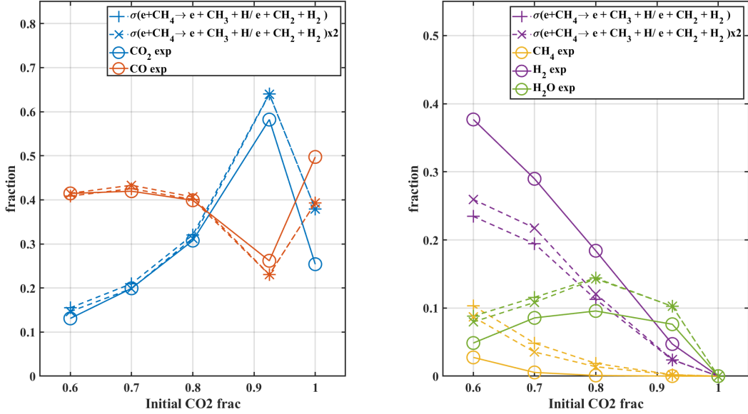
Figure 13: Study of the effect of the doubling of the CH 4 dissociation cross-section (taken from [44]) on the main products fractions at 1.85 sccm, 5 Torr. The experiment is plotted in plain lines, the simulation using the cross-section from [44] is plotted in dashed lines with + markers and the simulation with the cross-section doubled in dashed lines with x markers.
