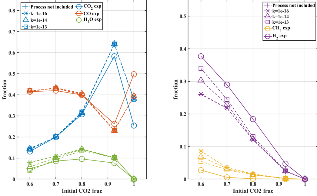
Figure 14: Study of the effect of the addition of process (14) on the main products fractions at 1.85 sccm, 5 Torr with different rate coefficient in \text{m}^3\text{s}^{-1} . The simulation is plotted in dashed lines and the experiment in plain lines
