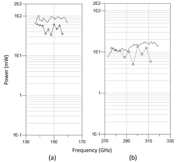
Figure 12: (a) Measured input powers before the 150 GHz thermal break titanium waveguide (300K: bold-light, 150K: bold-circle), (b) Measured and simulated power at 300 GHz (300K measurement: bold-light, 150K simulation: bold-circle).
