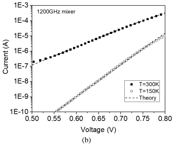
Fig. 11. IV characteristics measured (a) on 600 GHz doubler and (b) on 1200 GHz mixer at 150K (white squares) and 300 K (black squares). The dashed line is the theoretical fit [19][38].
