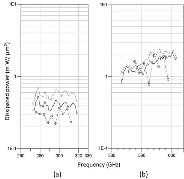
Figure 13: Dissipated power per anode area in \text{mW per } \mu\text{m}^2 for the (a) 300 GHz doubler and (b) 600 GHz doubler (300K measurement: bold-light, 300K simulation: dot-light, 150K simulation: dot with circle).
